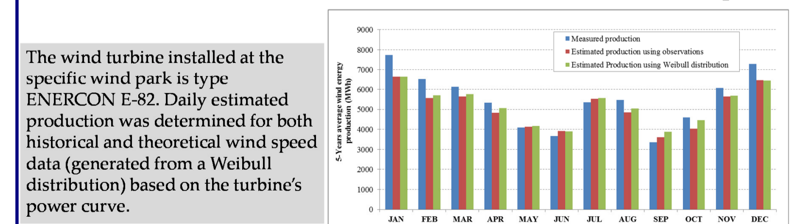
The wind turbine installed at the specific wind park is type ENERCON E-82. Daily estimated production was determined for both historical and theoretical wind speed data (generated from a Weibull distribution) based on the turbine's power curve.
