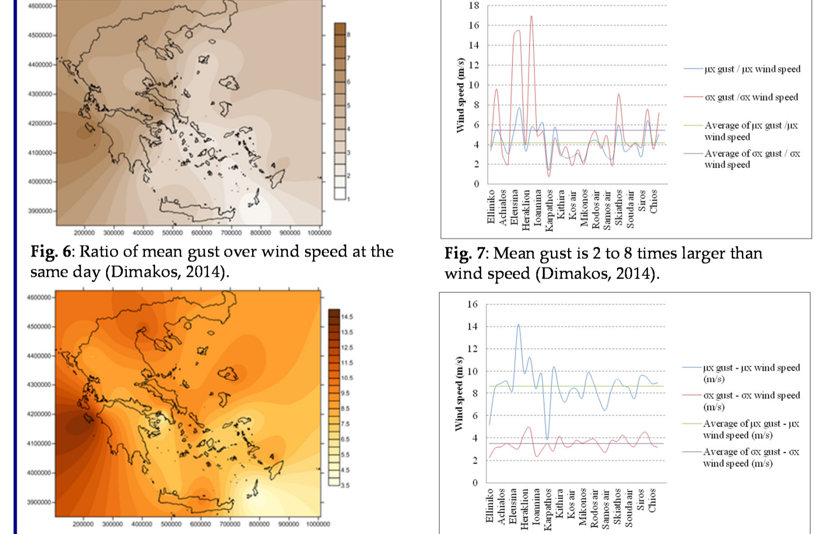
Fig. 6: Ratio of mean gust over wind speed at the same day (Dimakos, 2014).
