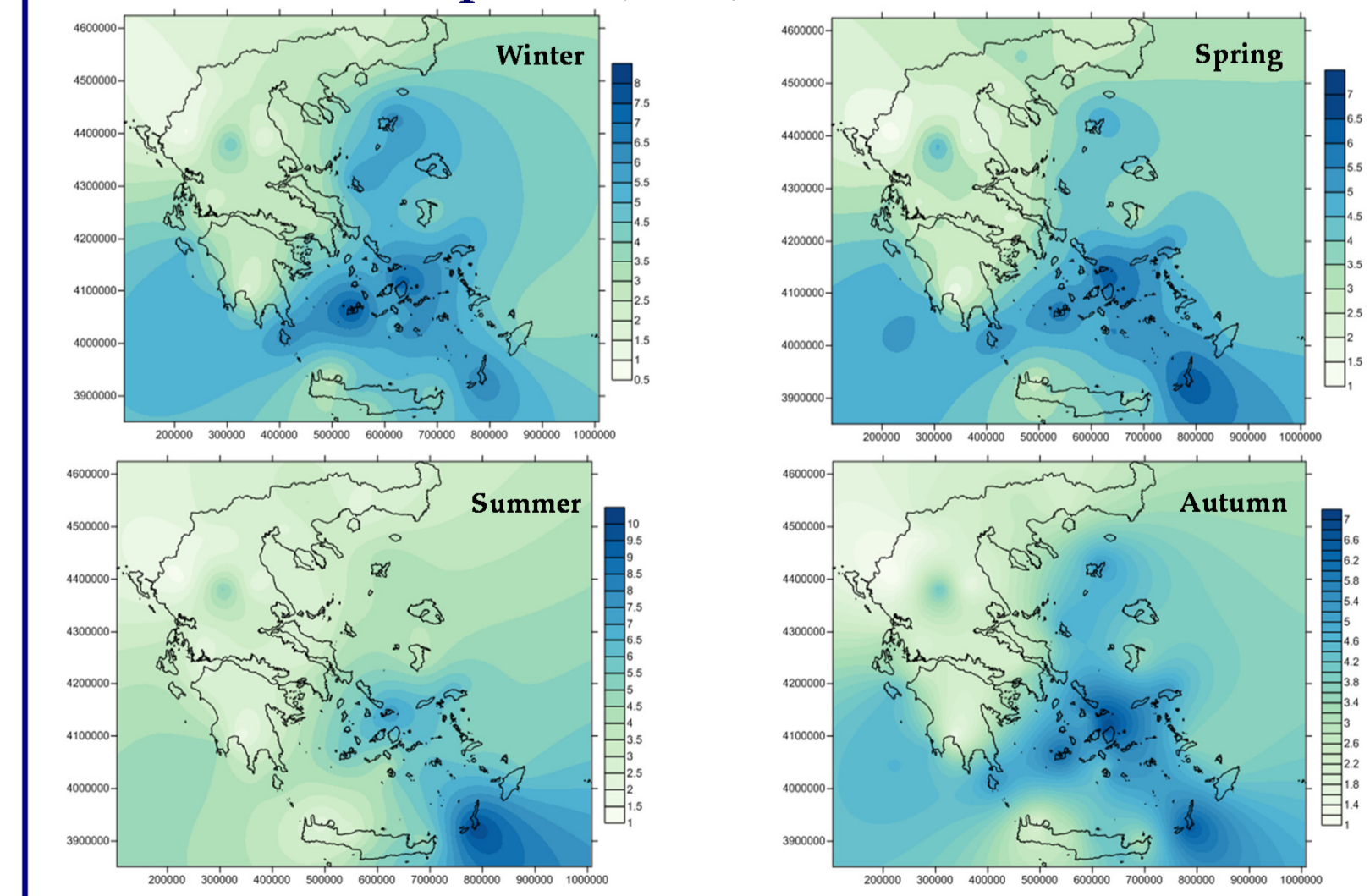
Fig. 3: Seasonal mean wind speed (m/s), over Greece (Dimakos, 2014).
