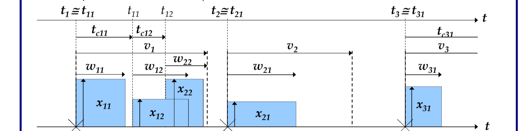
Fig. 13: Mathematical scheme describing the implemented modified Bartlett-Lewis model (Dimas, 2013).
