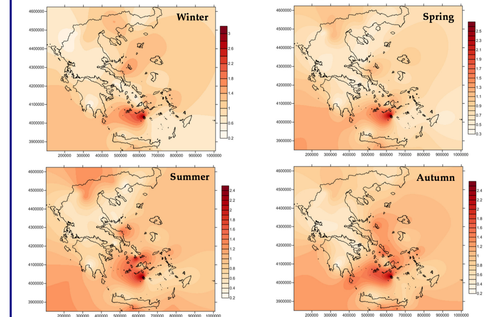
Fig. 4: Seasonal standard deviation of wind speed (m/s), over Greece (Dimakos, 2014).
