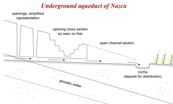
Sketch of the underground aqueduct
