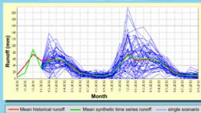
Runoff scenarios into the Moros reservoir
