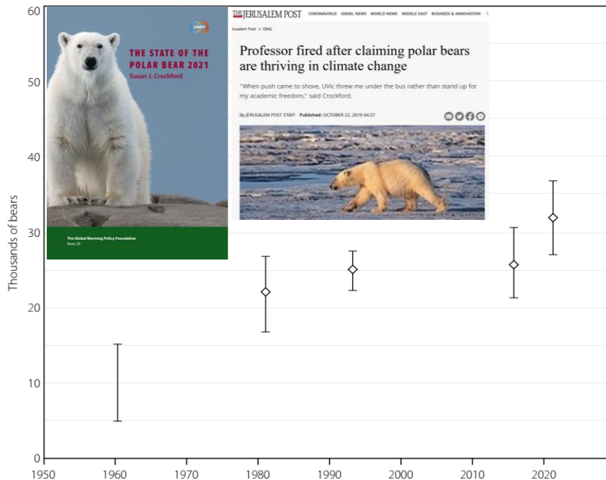
Figure 1: Estimates of the global polar bear population, 1960 to date.
