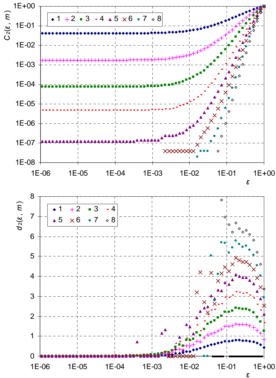
Figure 4 Correlation sums C_2(\varepsilon, m) (upper panel) and their local slopes d_2(\varepsilon, m) (lower panel) vs. scale \varepsilon for embedding dimensions m = 1 to 8 calculated from a series of 10 000 independent random values, 80% of which are generated from the uniform distribution and the remaining are zeros (located at random).
