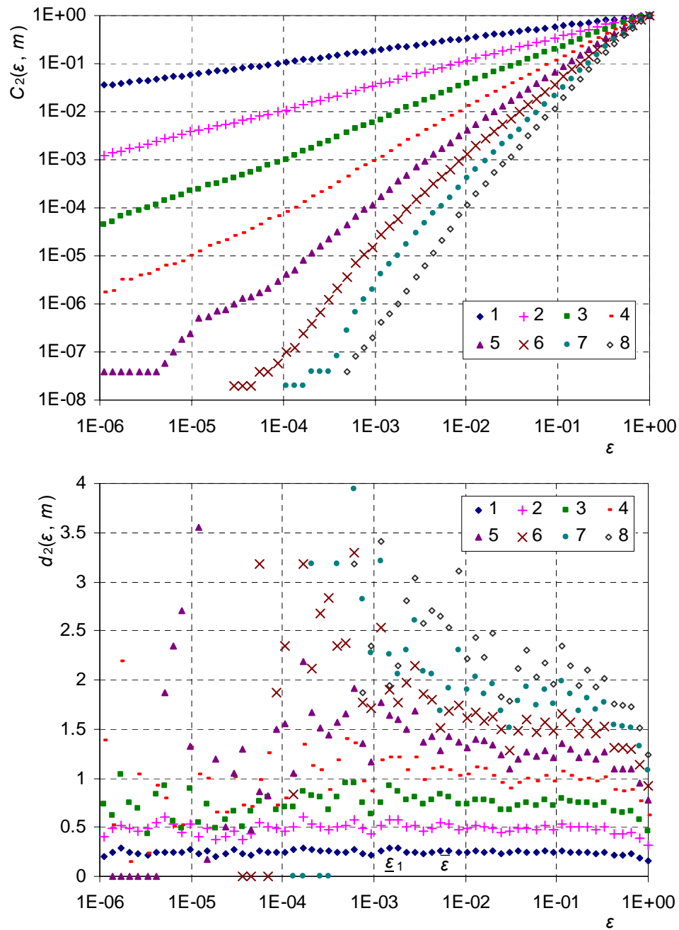
Figure 3 Correlation sums C_2(\varepsilon, m) (upper panel) and their local slopes d_2(\varepsilon, m) (lower panel) vs. scale \varepsilon for embedding dimensions m = 1 to 8 calculated from a series of 10 000 independent random values with Pareto distribution with exponent 1/8 .
