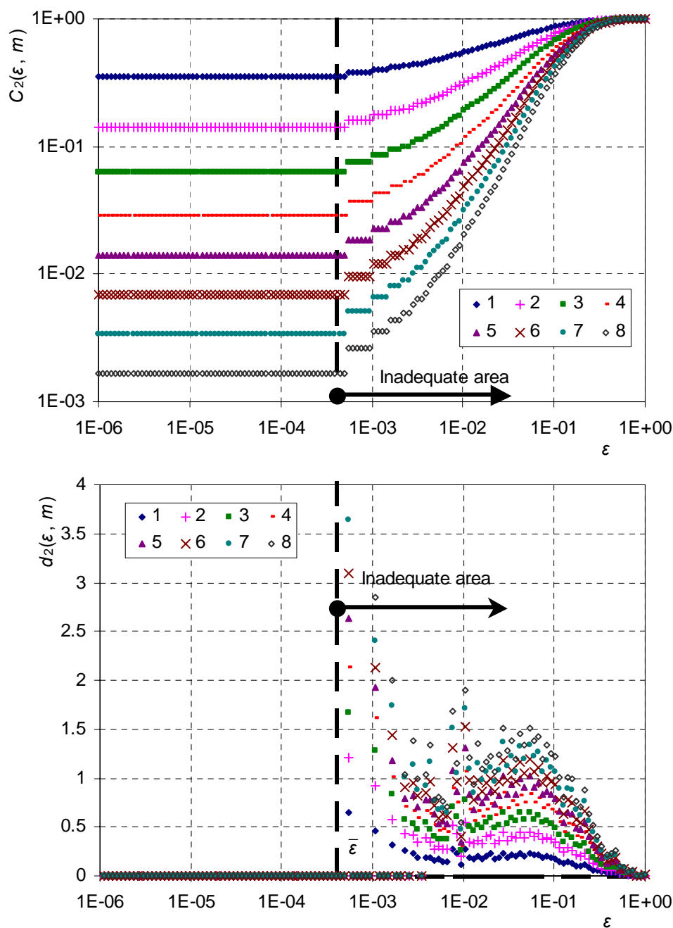
Figure 8 Correlation sums C_2(\varepsilon, m) (upper panel) and their local slopes d_2(\varepsilon, m) (lower panel) vs. scale \varepsilon for embedding dimensions m = 1 to 8 calculated from the daily rainfall series at the Vakari raingauge.
