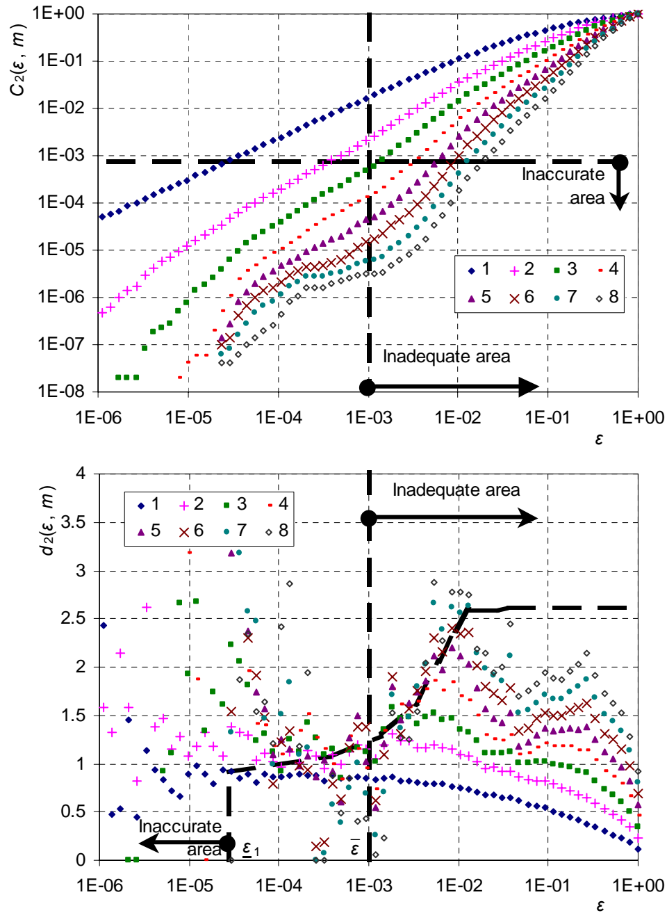
Figure 6 Correlation sums C_2(\varepsilon, m) (upper panel) and their local slopes d_2(\varepsilon, m) (lower panel) vs. scale \varepsilon for embedding dimensions m = 1 to 8 calculated from a series of 10 000 autocorrelated random values having approximately Pareto distribution with shape parameter 0.44.
