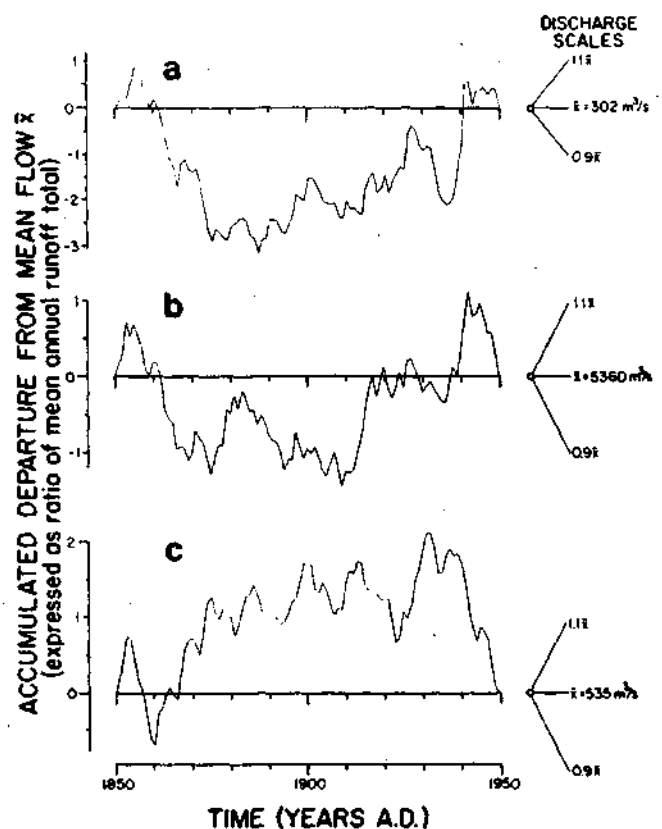
FIGURE 8.1 Accumulated departures from 100-yr mean flow \bar{x} (1851-1950) for three European rivers (mean flow for any intervening period is given by the slope of a straight line connecting its endpoints projected on the curve; it can be measured by the discharge scale shown). a, Elbe, Decin, Czechoslovakia; b, Danube, Orshava, Romania; c, Gota, Sjotorp Vanersbury, Sweden (Data sources: a, Novotny, 1963; b and c, Yevjevich, 1963).
