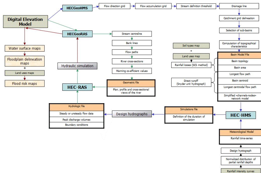
Figure 2. Interactive geomorphologic, hydrological and hydraulic processes in floodplain inundation design (Gkiokas, A., 2009)
