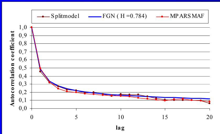
Autocorrelogram of annual discharge time series
