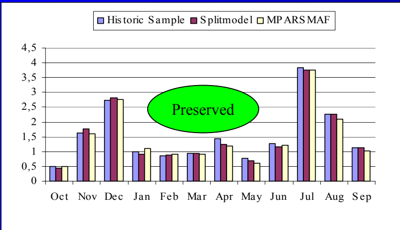
Monthly skewness coefficients of discharge time series
