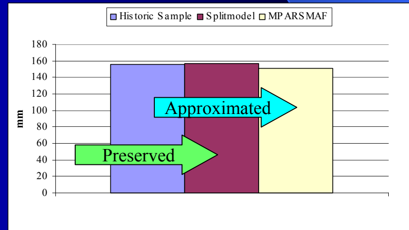
Annual standard deviation of rainfall time series
