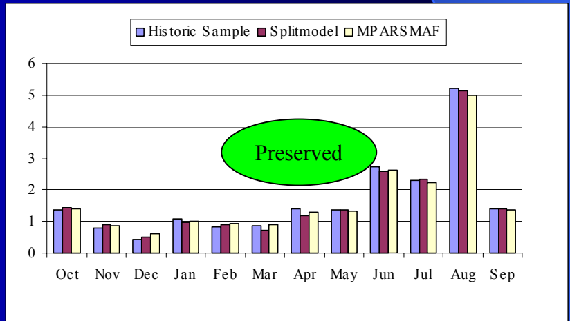
Monthly skewness coefficients of rainfall time series
