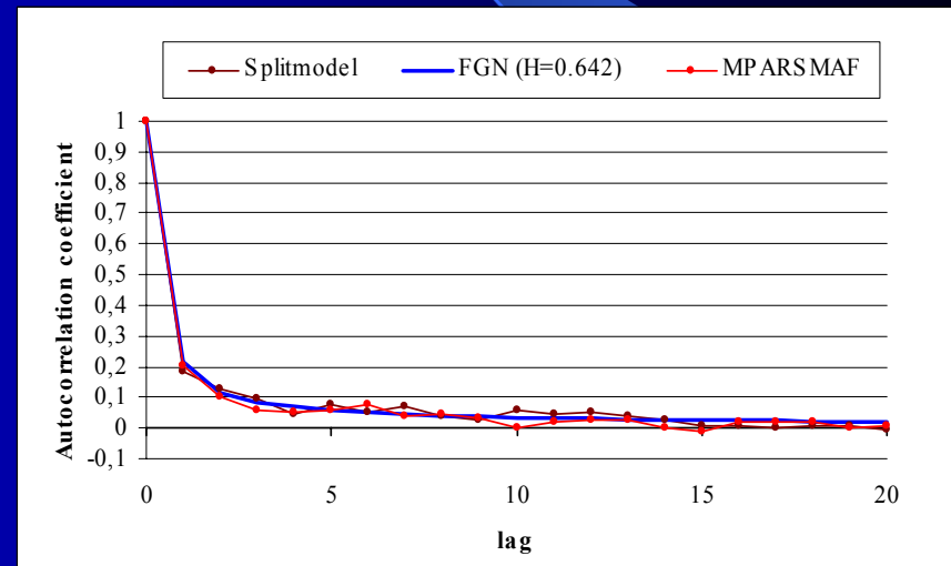
Autocorrelogram of annual rainfall time series
