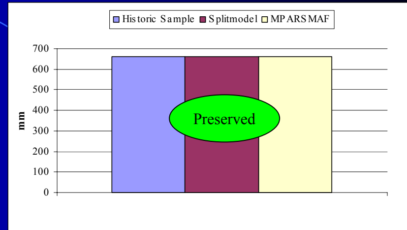
Annual expected value of rainfall time series
