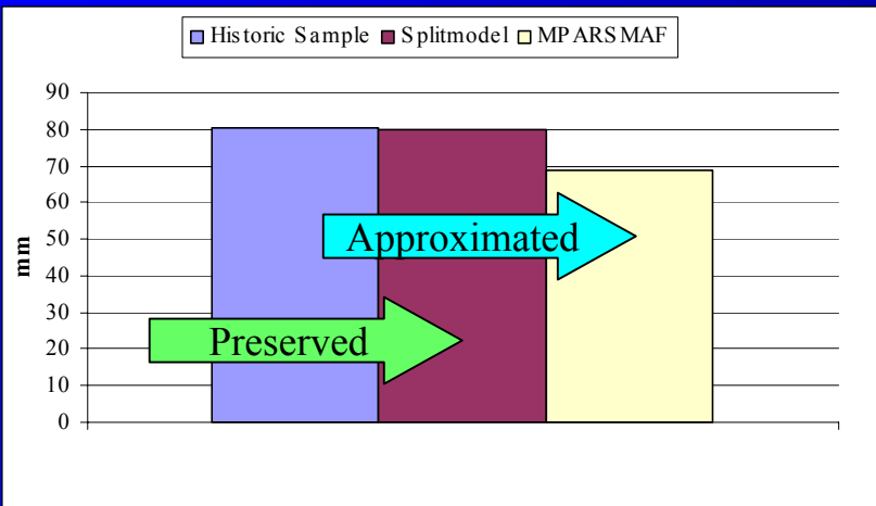
Annual standard deviation of discharge time series
