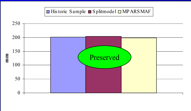
Annual expected value of discharge time series
