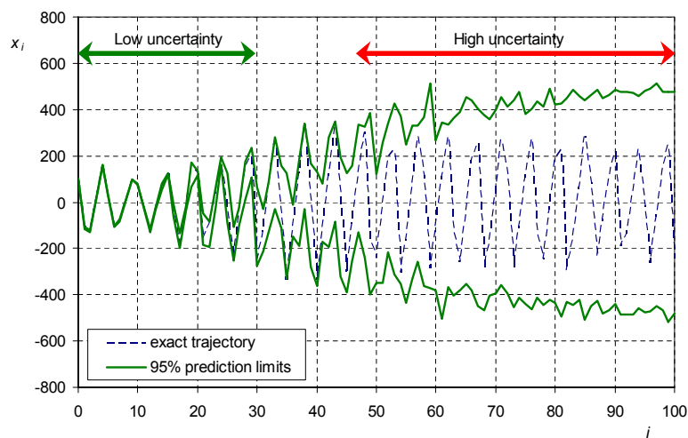
Fig. 8. Stream tube representation of the evolution of soil water x (with initial conditions as in Fig. 4 and 1% uncertainty) in a stochastic setting using Monte Carlo prediction limits for 95% probability of bracketing the true state between the stream tube “walls” (1000 simulation runs).
