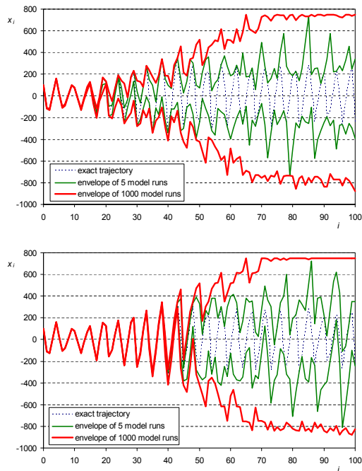
Fig. 6. Stream tube representation of the evolution of soil water x (with initial conditions as in Fig. 4 and 1\% uncertainty) in a deterministic setting using envelope curves: (upper) when only x_0 is observed; (lower) when x_0 to x_{30} are observed.
