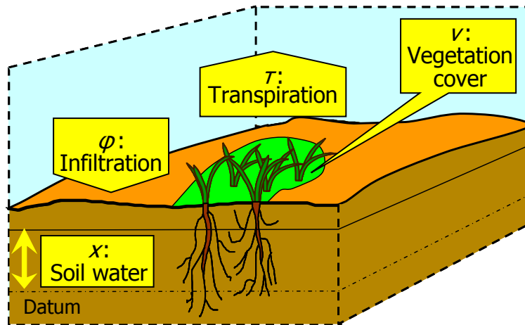
Fig. 1. A caricature hydrological system for which the toy model was constructed.
