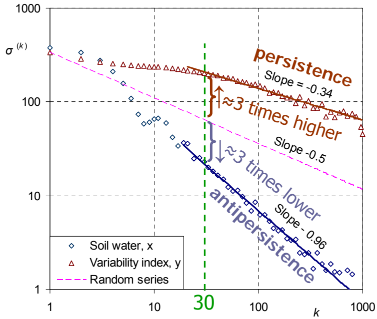
Fig. 15. Climacograms (plots of standard deviation \sigma^{(k)} vs. averaging scale k ) of the time series x_i and y_i (where standard deviations were estimated by the classical statistical estimator of time series averaged on each scale k ).
