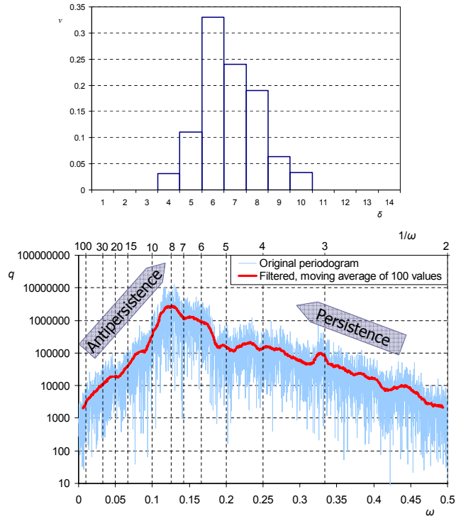
Fig. 13. Graphical depiction of periodic properties of the system based on (upper) a histogram of the time between successive peaks, \delta , of the soil water x_i , where \nu is the fraction of occurrences of a certain \delta over the total number of occurrences; (lower) the periodogram of the time series of x_i , where \omega is frequency and q the spectral density; 10 000 terms of time series were used for the construction of the plots.
