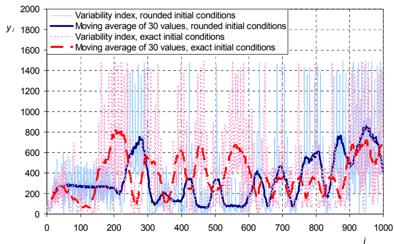
Fig. 16. Plot of 1000 terms of the time series y_i (variability index) at scales 1 and 30 and for two sets of initial conditions differing less than 1%.
