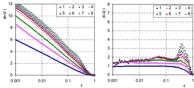
Fig. 11. Graphical depiction of the application of the algorithm to recover the system dynamics (with emphasis of its dimensionality) from time series of 10 000 points.
