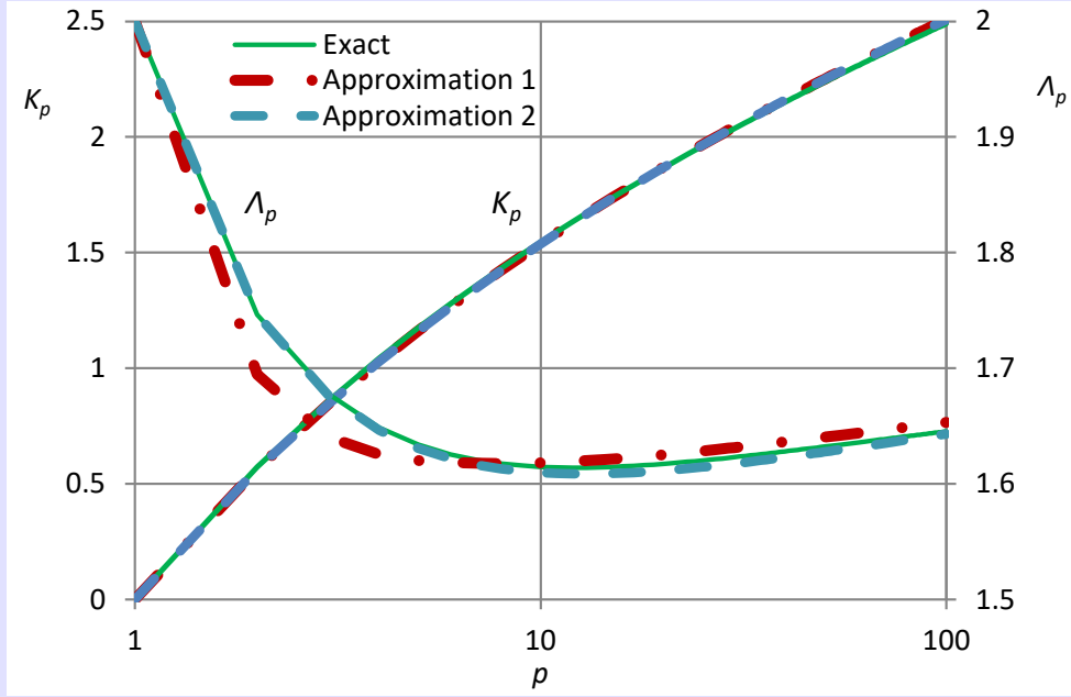
Figure 6.25 Comparison of approximate and exact values of K-moments and \Lambda -coefficients for the normal distribution. Approximations 1 and 2 are calculated by equations (6.161) and (6.163), respectively, and the exact values are calculated by numerical integration.
