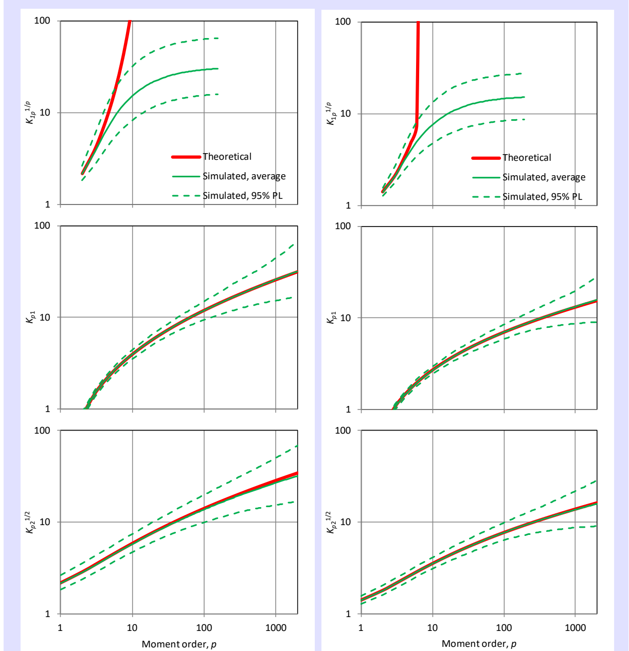
Figure 6.7 Illustration of the performance of the K-moment estimator of equations (6.60)–(6.62), applied to upper central K-moments, for the lognormal distribution ( left column ; \text{LN}(0,1) ) and the Pareto distribution ( right column ; upper-tail index \xi = 0.15 scale parameter \beta = 1 , lower bound zero) for q = 1 ( middle row ) and q = 2 ( bottom row ). For comparison, the performance of the estimators of classical moments is also shown ( upper row ; notice that in the Pareto distribution the true moments are \infty for p > 1/0.15 = 6.87 ). The true moments were determined by numerical integration for the lognormal distribution and from the equations in Table 6.2 for the Pareto distribution. The estimates are averages of 100 simulations each with n = 2000 and are indistinguishable from the true (theoretical) values. The 95% prediction limits (PL) are also shown.
