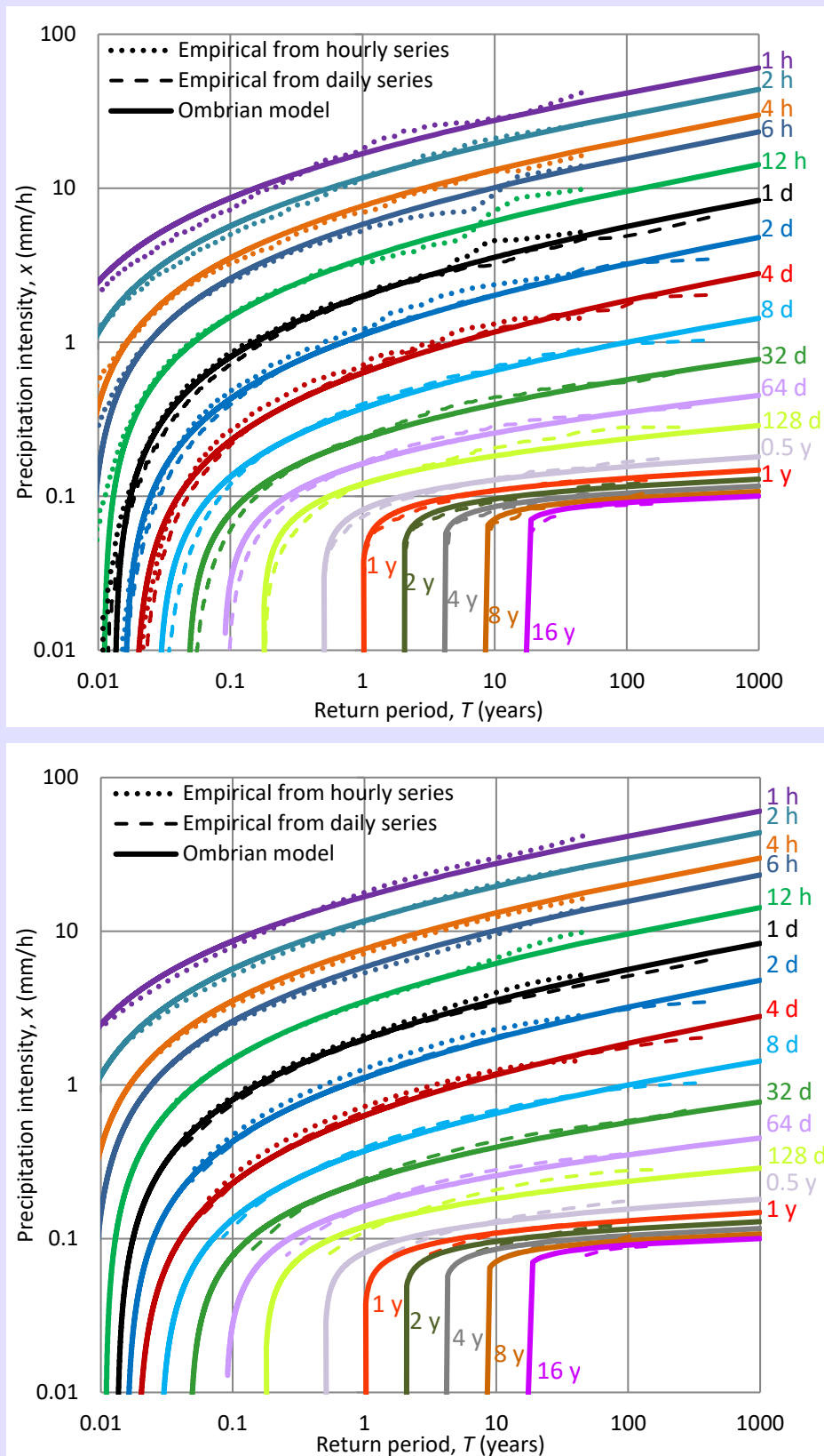
Figure 8.8 Ombrian curves as resulted from the ombrian model for Bologna for time scales spanning 5 orders of magnitude (1 h to 16 years = 140256 h). The empirical points are estimated from ( upper ) order statistics (using formula VII of Table 5.5) and ( lower ) K-moments. In both cases the effect of persistence was taken into account; the ombrian model results were plotted for bias-adapted variance in order to be comparable with empirical plots (thus, for k > 1000 h or about 40 d, the true intensity resulting from the model is higher than what is shown in the graph). The abbreviation “y” stands for year.
