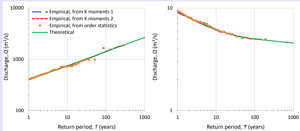
Figure 9.4 Comparison of empirical and theoretical (PBF) distributions fitted on daily data of the French Broad River at Asheville, NC, USA, as in Figure 9.3 but with a fitting on T > 1 year ( left ) or \bar{T} > 1 year ( right ). The parameters are, for the left panel: \xi = 0.277, \zeta = 5.06, \lambda = 81.7 \text{ m}^3/\text{s}, x_L = 4.87 \text{ m}^3/\text{s} , and for the right panel: \xi = 0, \zeta = 2.16, \lambda = 77.3 \text{ m}^3/\text{s}, x_L = 4.40 \text{ m}^3/\text{s} .
