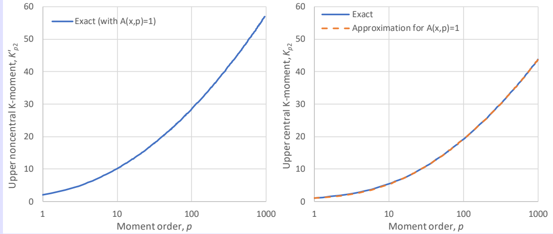
Figure 6.5 Comparison of exact upper K-moments of orders p, 2 and approximations thereof setting A(x, p) = 1 , for the exponential distribution with mean 1; ( left ) noncentral and ( right ) central upper K-moments. (Source: Koutsoyiannis, 2023).
