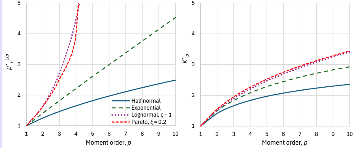
Figure 6.1 Increase of (left) classical moments and (right) K-moments with the increase of moment order p for the indicated distributions, all of which are defined on [0, \infty) and have mean 1.
