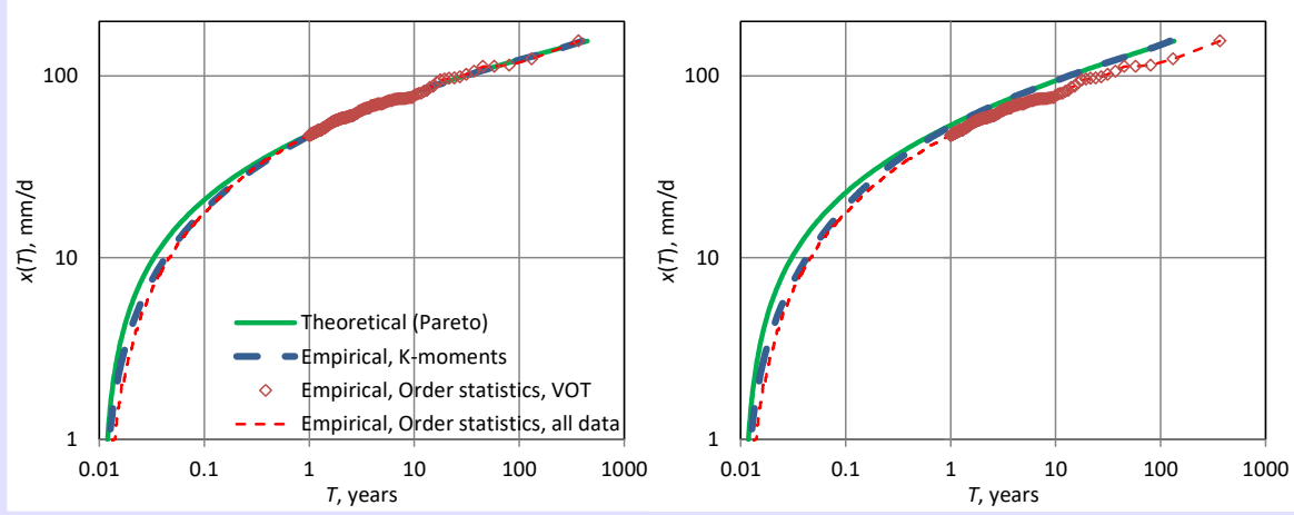
Figure 6.32 Probability plot (in terms of quantile x vs. return period T ) showing the fitting of the Pareto distribution on the Bologna daily rainfall record by the indicated methods, (left) assuming independence and (right) accounting for long-range dependence; the curves of theoretical and empirical K-moments are indistinguishable for T > 1 year. The empirical distribution from order statistics (calculated by formula IV of Table 5.5 and not considering dependence so that it is the same in both panels) is also plotted for comparison.
