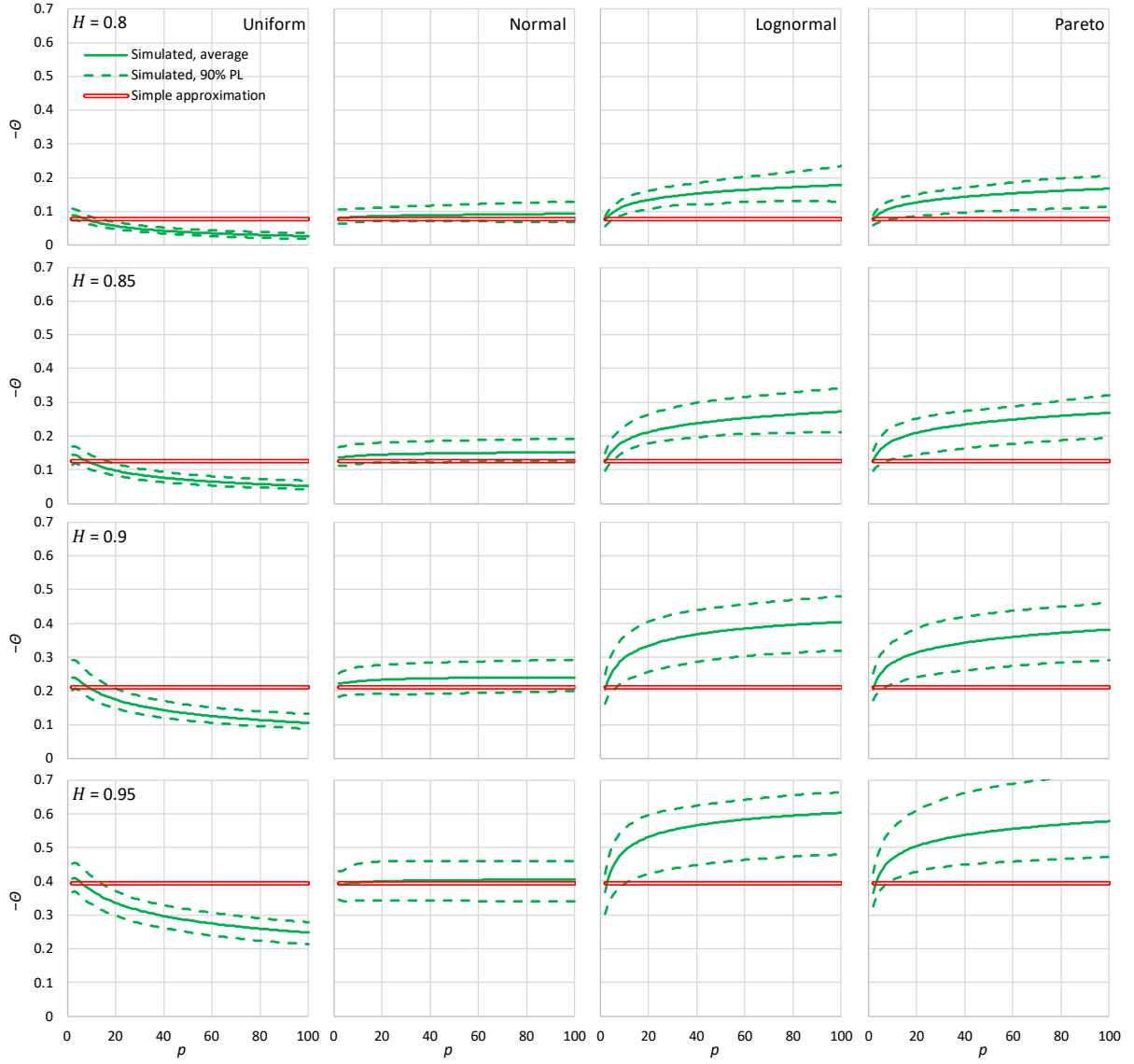
Figure 6.38 Results of Monte Carlo simulations to determine the relative bias, \theta(n, p) for the indicated values of the Hurst parameter H and the indicated distributions. The ‘simple approximation’ corresponds to equation (6.134). For the details of the simulation see text.
