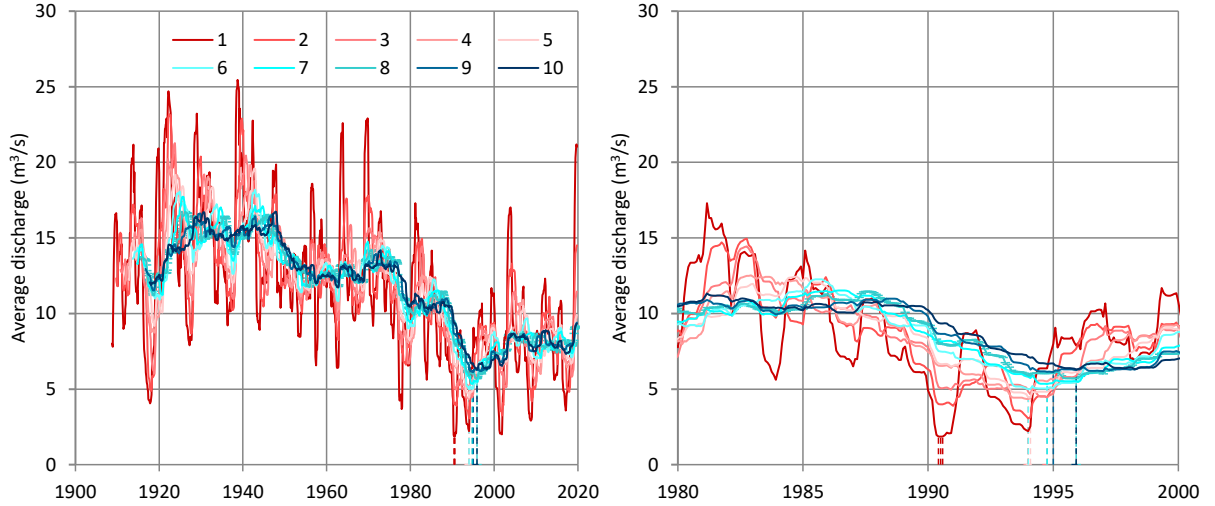
Figure 1.9 (left) Plot of the (right-aligned) moving average of the Boeotikos Kephisos discharge for the time scales noted in the legend; the time locations of the observed minima at each scale are also shown with dashed lines of the same colour as the corresponding moving-average time series. (right) Close up of the left panel for years 1980-2000.
