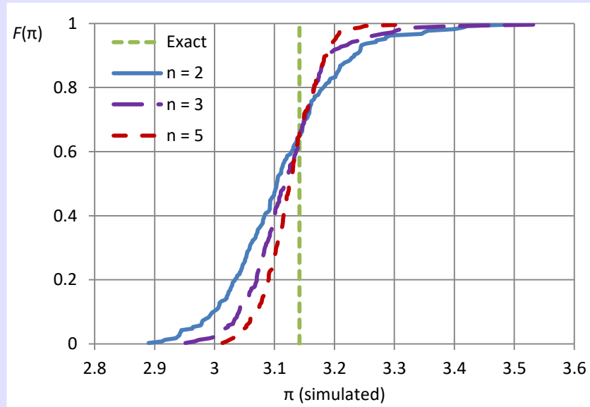
Figure 5.12 Simulation results to estimate \pi from m = 100\,000 random samples, each consisting of n random numbers from the Pareto distribution with upper-tail index \xi = 0.5 . The curves depict the sampling distributions of \pi estimates for the indicated three values of n .
