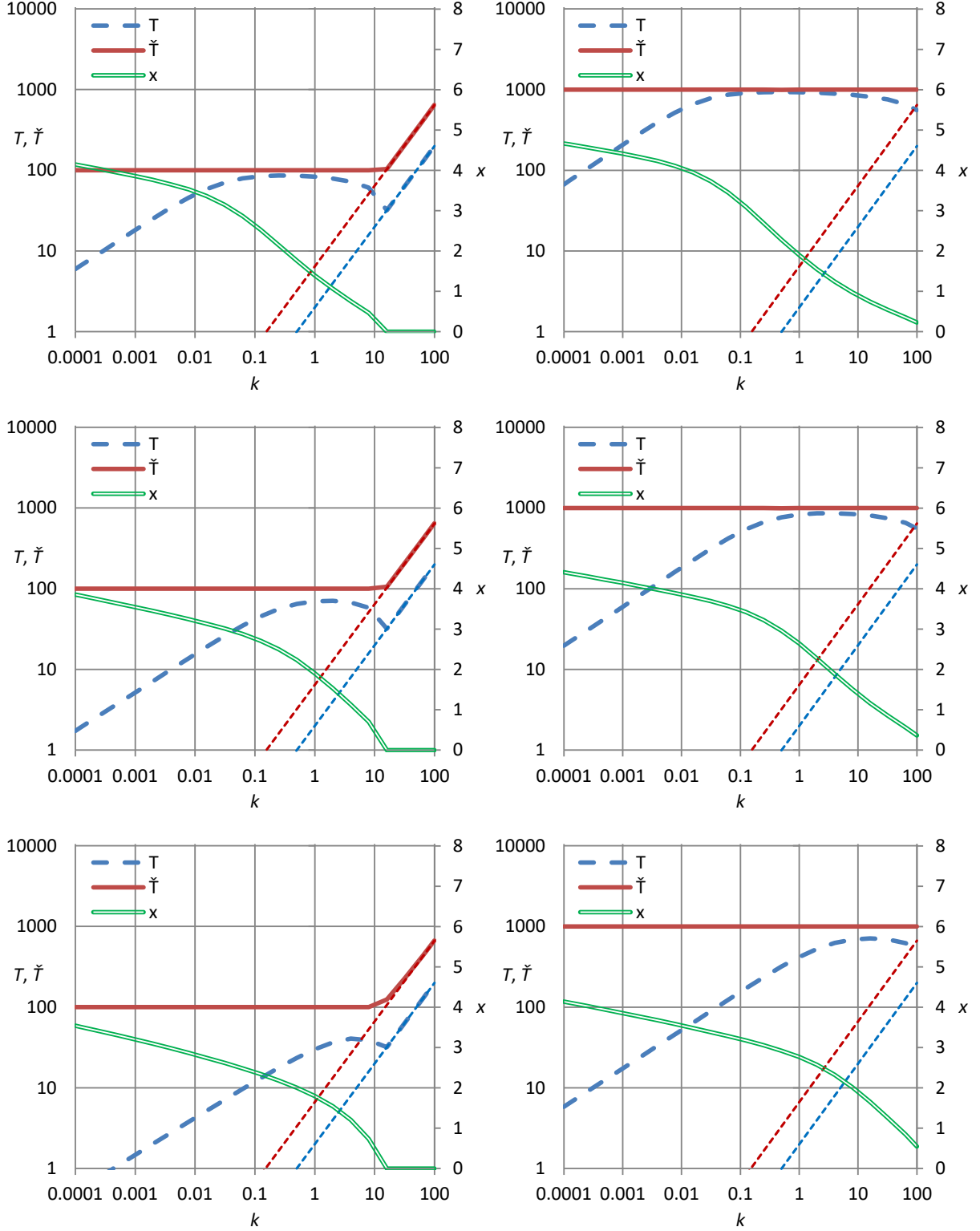
Figure 5.9 Illustration of the variation of the threshold value x^{(k)} and the return period T^{(k)} vs. the time scale k for constant \tilde{T}^{(k)} = 100 (left column) and \tilde{T}^{(k)} = 1000 (right column) and for a neutral FHK-C process with standard normal distribution for the instantaneous process ( \lambda = 1 ), M = 0.5 , H = 0.8 and \alpha = 0.1 (close to pure randomness; upper row), \alpha = 1 (middle row) and \alpha = 10 (high short-range dependence; lower row). Dotted lines represent the lowest feasible values of T^{(k)} and \tilde{T}^{(k)} , when P_1 = 0.5 and x = 0 .
