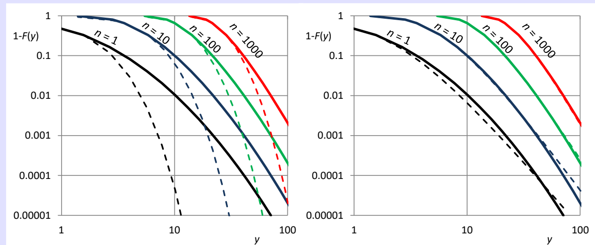
Figure 2.9 Approximation of the true distribution of the maximum of n independent variables with lognormal distribution \text{LN}(0,1) (continuous lines) by the limiting extreme value distribution (dashed lines), which is (left) EV1 and (right) EV2 with \xi = 0.3/n^{0.07} , which was found after a numerical investigation and fitting a power function of n by minimizing the fitting error.
