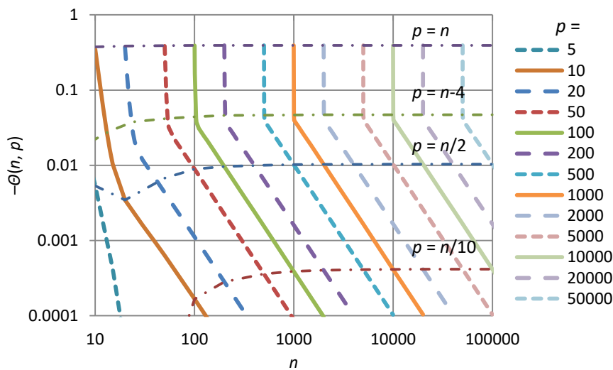
Figure 6.37 Deviation -\theta(n, p) in fulfilling the necessary unbiasedness condition (6.59) of the estimator (6.273), as a function of sample size n and K-moment order p . Dash-dot lines correspond to the specified values of p as fractions of n .
