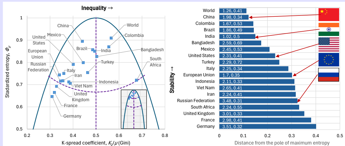
Figure 6.17 Characteristic graphs for large population countries with data availability in 2022 (except South Africa, in which the most recent data are for 2017): (left) standardized entropy vs. K-spread coefficient (Gini index), plotted alongside the maximum entropy vs. K-spread curve; (right) distance from the pole of maximum entropy, where the lower-tail index \zeta and the upper-tail index \xi are noted in each country's bar, while five major geopolitical players are flagged. The inset in the left graph contains the entire range as in Figure 6.16 and purple dashed lines show the boundaries between the partitioned areas. (adapted from Koutsoyiannis and Sargentis, 2026.)
