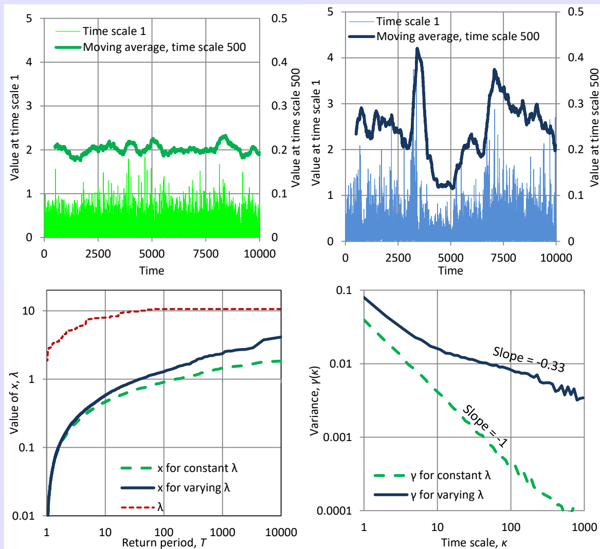
Figure 3.9 Graphs for the hypothetical example studied in Digression 3.I: ( upper left ) for constant \lambda ; ( upper right ) for varying \lambda ; ( lower left ) plots of distribution functions; ( lower right ) plots of climacograms (see text for further explanation).
