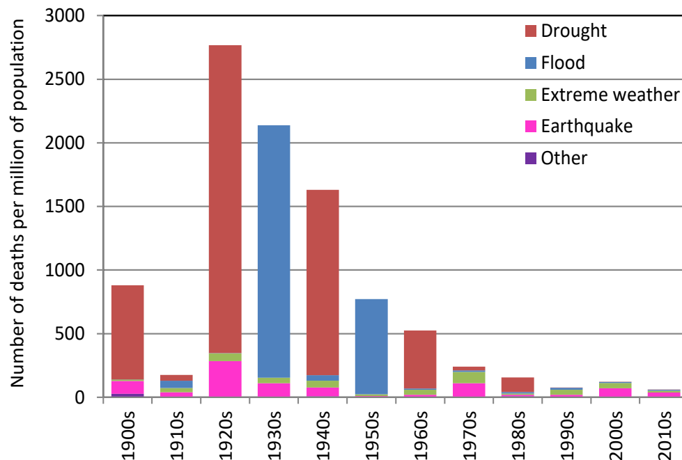
Figure 11.14 Evolution of the frequency of deaths from natural disasters per decade in the 20 th and 21 st century. In addition to deaths from floods and droughts, deaths from other categories of natural catastrophes are also plotted: “extreme weather” includes storms, extreme temperatures (cold- or heatwave, severe winter conditions) and fog; “earthquake” also includes tsunamis; “other” comprises landslides (wet or dry), rockfalls, volcanic activity (ash fall, lahar, pyroclastic flow and lava flow) and wildfires. (Source: Koutsoyiannis, 2020b; victim data: OFDA/CRED International Disaster Database * ; population data: United States Census † .)
