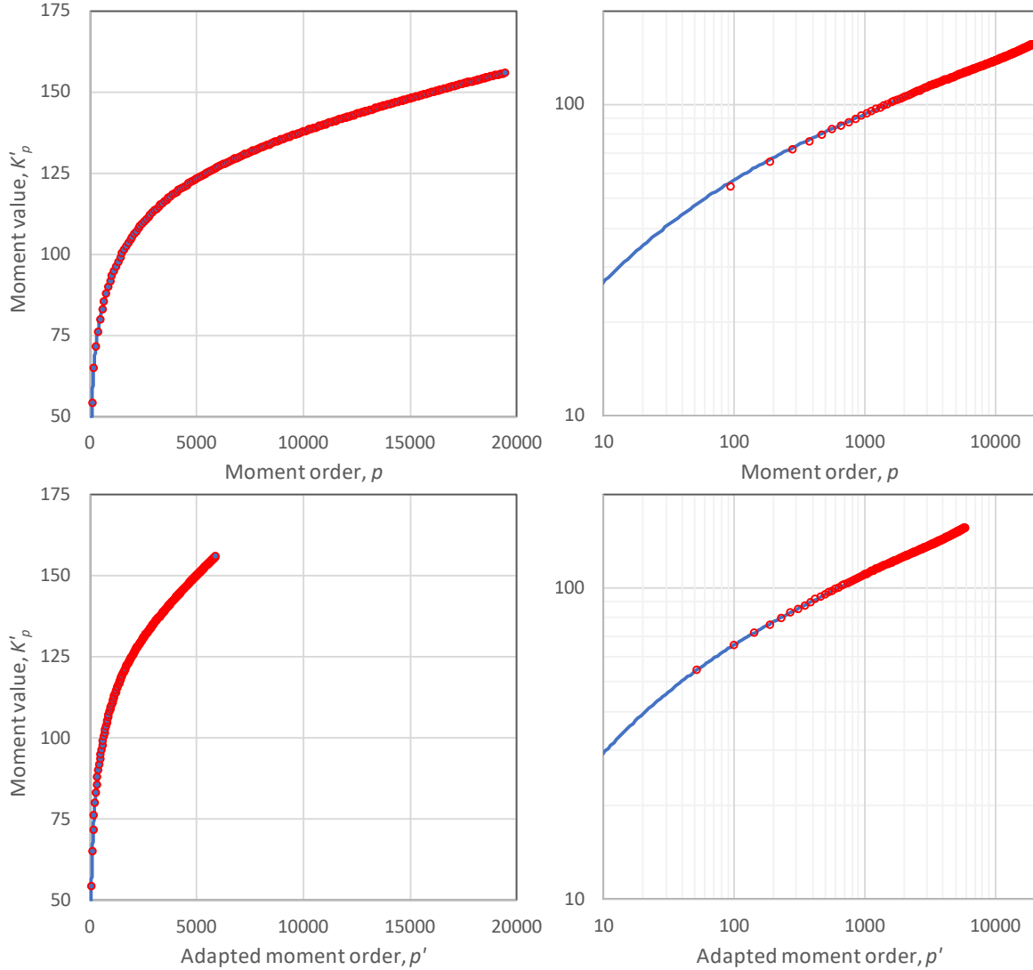
Figure 6.35 Verification, using the daily precipitation data of Bologna, of the correspondence of K-moments estimated from block maxima (206 annual maxima) by equation (6.186) with the K-moments of the original process: (left column) Cartesian axes; (right column) logarithmic axes; (upper row) original moment orders, neglecting dependence and using equation (6.185); (lower row) adapted moment orders, after considering long-term dependence ( H = 0.9 ) and using equation (6.186).
