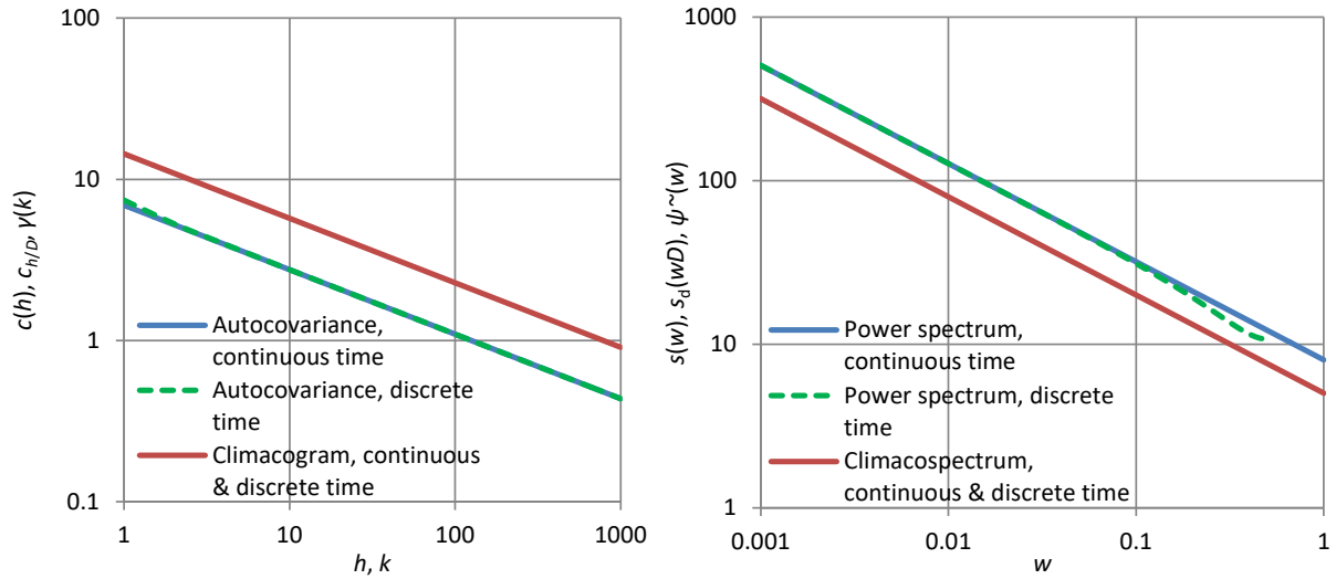
Figure 3.6 Second-order characteristics of a HK process with parameters \lambda = 1 , \alpha = 20 , H = 0.8 and discretization time step D = 1 . The climacogram and climacospectrum are precisely the same for the continuous- and discrete-time representations. The autocovariance and the power spectrum have some differences between the two representations, which are visible in both cases.
