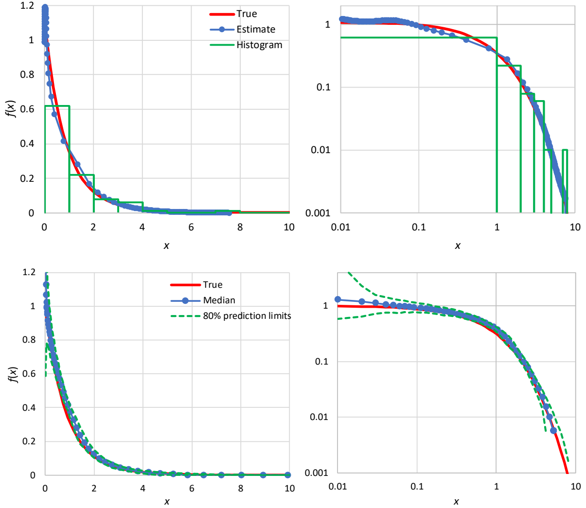
Figure 6.36 Illustration of the probability density estimate using the K-moment framework with a Pareto distribution with mean \mu = 1 and upper-tail index \xi = 0.1 , plotted in (left column) Cartesian and (right column) logarithmic axes. (upper row) Simulation results from a single data series of n = 100 values generated from the Pareto distribution. The points marked as “estimate” are calculated by equation (6.188) and their abscissae are the midpoints of the intervals (\hat{K}'_p, \hat{K}'_{p+1}) and (\hat{\hat{K}}'_{p+1}, \hat{\hat{K}}'_p) . For comparison, the histogram of 10 bins, calculated by the standard method for the range [0, 10] (width w = 2 ) is also shown. (lower row) Simulation results from 100 data series of n = 100 values each, processed to calculate the median of the estimates and produce their uncertainty band in terms of prediction limits, where the original results (whose abscissae differ in the different series) are interpolated at the points that are plotted in the graphs.
