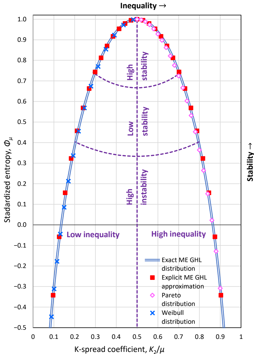
Figure 6.16 Maximum entropy vs. K-spread curve: maximum standardized entropy \Phi_\mu that is feasible for a specified K-spread coefficient K_2/\mu . A particular state, defined as a point (K_2/\mu, \Phi_\mu) is feasible only if it lies below this curve. The exact curve corresponds to the generalized half logistic (GHL) distribution, while different approximations (practically indistinguishable from the exact curve) are also plotted. Purple dashed lines show the boundaries between the partitioned areas.
