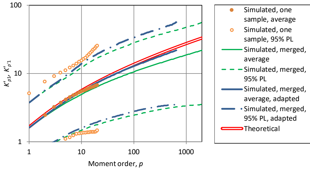
Figure 6.26 Illustration of the performance of the adaptation of K-moment estimation for a merged time series composed of m = 100 correlated time series of size n_1 = 20 each, generated from the exponentiated HK process for H = 0.8 , having lognormal marginal distribution (LN(0,1)) . The correlation of the logarithms of the variables of the different time series (which have normal distribution) is r = 0.64 . The K-moments shown are noncentral for q = 1 . For comparison, estimates from one time series with size n_1 = 20 are also shown. All estimates are averages of 100 simulations, while 95% prediction limits (PL) are also shown.
