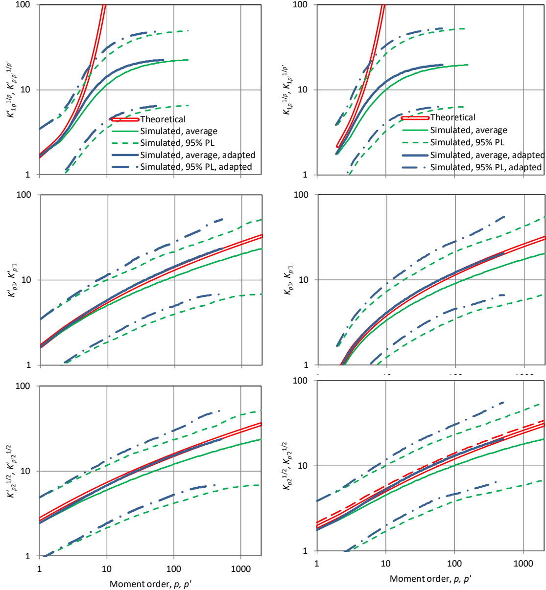
Figure 6.23 Illustration of the performance of the adaptation of K-moment estimation for an HK process with Hurst parameter 0.9 and lognormal marginal distribution (LN(0,1); same as in Figure 6.7, left): (left column) noncentral moments; (right column) central moments; (middle row) q = 1 (bottom row) q = 2 . For comparison classical moments are also shown (upper row) . The estimates are averages of 200 simulations each with n = 2000 and are almost indistinguishable from the theoretical values. The first-order approximation of equation (6.133) was used for the adaptation. For K_{p2} (lower right) the true K-moments are represented by the dashed curve while the curve marked “theoretical” corresponds to the true plus bias, where bias is determined from equation (6.138). The 95% prediction limits (PL) are also shown.
