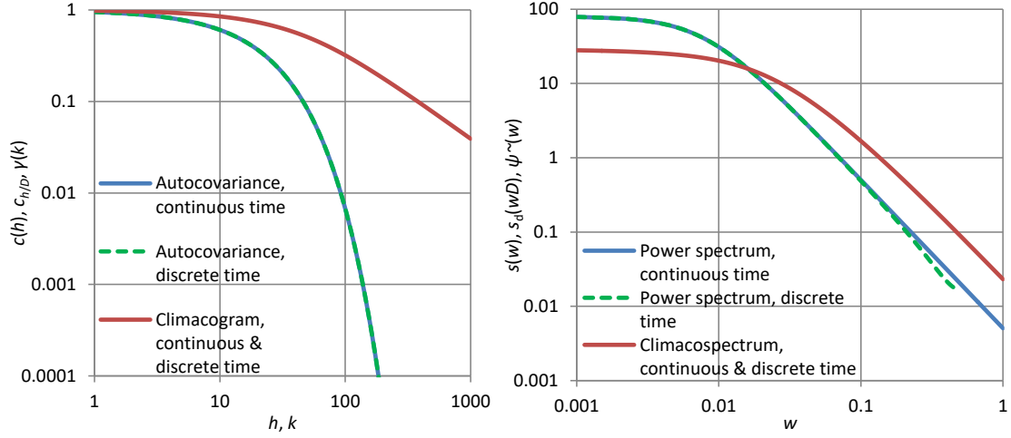
Figure 3.5 Second-order characteristics of a linear Markov process with parameters \lambda = 1 , \alpha = 20 and discretization time step D = 1 . The climacogram and climacospectrum are precisely the same for the continuous- and discrete-time representations. The autocovariance and the power spectrum have some differences between the two representations which are invisible in the former case and visible in the latter.
