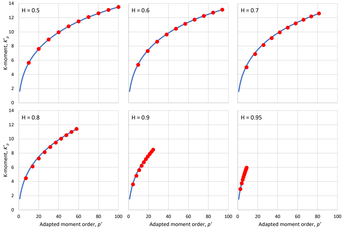
Figure 6.34 Stochastic simulation results for the correspondence of K-moments estimated from block maxima by equation (6.186) with the K-moments of the original process. The results are for an HK process with the indicated Hurst parameter H and lognormal distribution with shape parameter \zeta = 1 . The lines correspond to the original process whose K-moments were estimated as the averages of an ensemble of 100 simulations with length nb = 100 . The points correspond to the process of block maxima, estimated from the same simulations, after grouping the time series of 100 items into 10 blocks of length 10 each and taking the maxima of the blocks. The adapted moment order refers to the original process ( \underline{x}_t ). The case H = 0.5 (upper left) refers to a process with independence, for which equation (6.185) applies.
