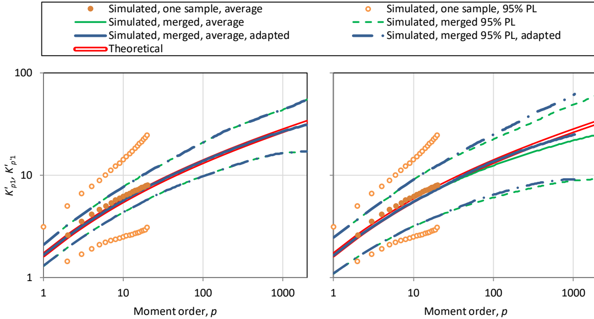
Figure 6.25 Illustration of the performance of the adaptation of K-moment estimation for a merged sample composed of m = 100 correlated sub-samples of size n_1 = 20 each. Each sub-sample is random with lognormal marginal distribution \text{LN}(0,1) ; same as in Figure 6.7, left). The correlation of the logarithms of the variables (which have normal distribution) are r = 0.25 ( left ) and r = 0.64 ( right ). The K-moments shown are noncentral for q = 1 . For comparison, estimates from one sample with size n_1 = 20 are also shown. All estimates are averages of 100 simulations, while 95% prediction limits (PL) are also shown. In the left graph ( r = 0.25 ) the adaptation turns out to be negligible and the adapted curves are indistinguishable from the non-adapted.
