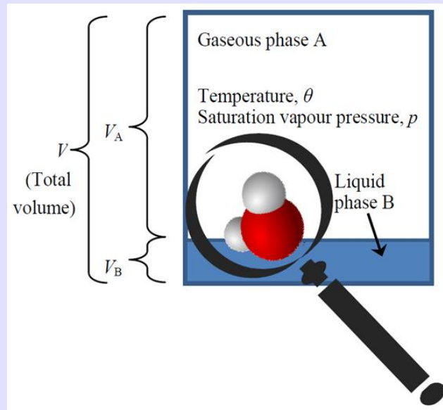
Figure 10.15 Explanatory sketch indicating basic quantities involved in the equilibrium of water vapour with liquid water, zooming in on a single “shy” molecule which “tries to hide itself” by maximizing the combined uncertainty \varphi related to its phase (being either gaseous or liquid with probabilities P_A and P_B , respectively), position and kinetic state.
