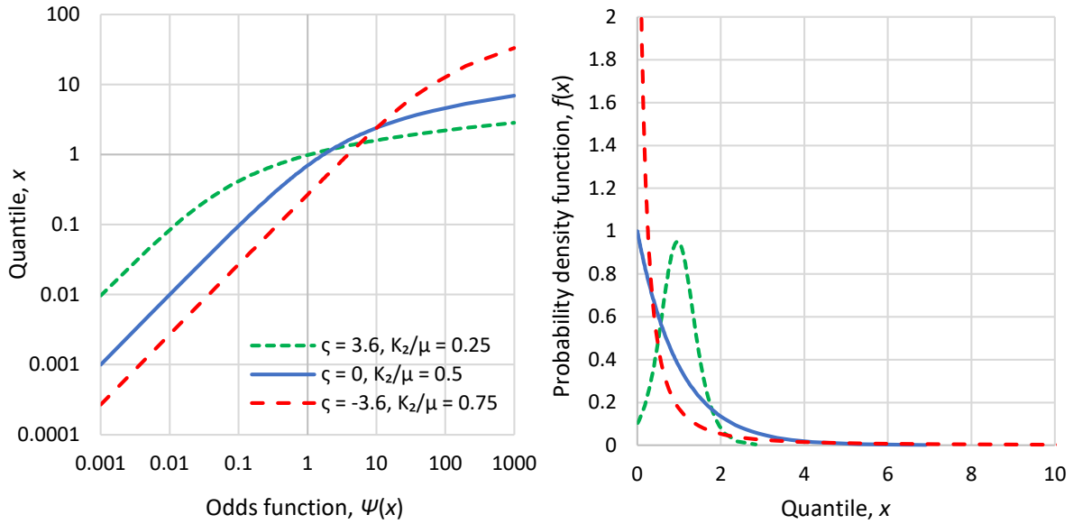
Figure 6.15 Probability plots of the GHL distribution for the indicated three parameter values, in terms of (left) quantile x vs. odds function \Psi(x) and (right) probability density function.
