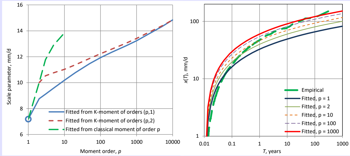
Figure 6.30 (left) Estimate of the scale parameter \lambda of the exponential distribution from the p th moment, fitted on the Bologna rainfall record; the circle corresponds to the standard estimate found by any of the methods of classical moments, L-moments, K-moments and maximum likelihood. (right) Resulting fitted distribution, as a graph of x vs. T , for the indicated values of p ; the empirical distribution is calculated by formula IV of Table 5.5.
