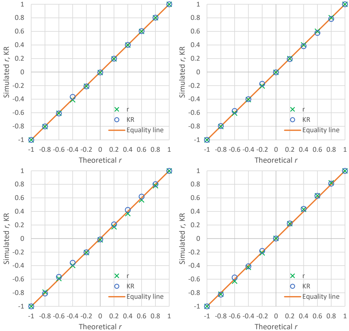
Figure 6.19 Simulation results of standard correlation ( r ) and K-correlation (KR) for a pair of stochastic variables linearly dependent, obtained by 10 000 generated pairs. The first variable in the pair has distribution, for the four panels seen clockwise: uniform, normal, lognormal with shape parameter \zeta = 1 , and Pareto with upper-tail index \xi = 0.25 . The second variable is a weighed sum of the first one and an auxiliary variable with distribution identical to that of the first, where the weights are such that the correlation between the first and the second variable be a specified value ('theoretical r ' in the graphs).
