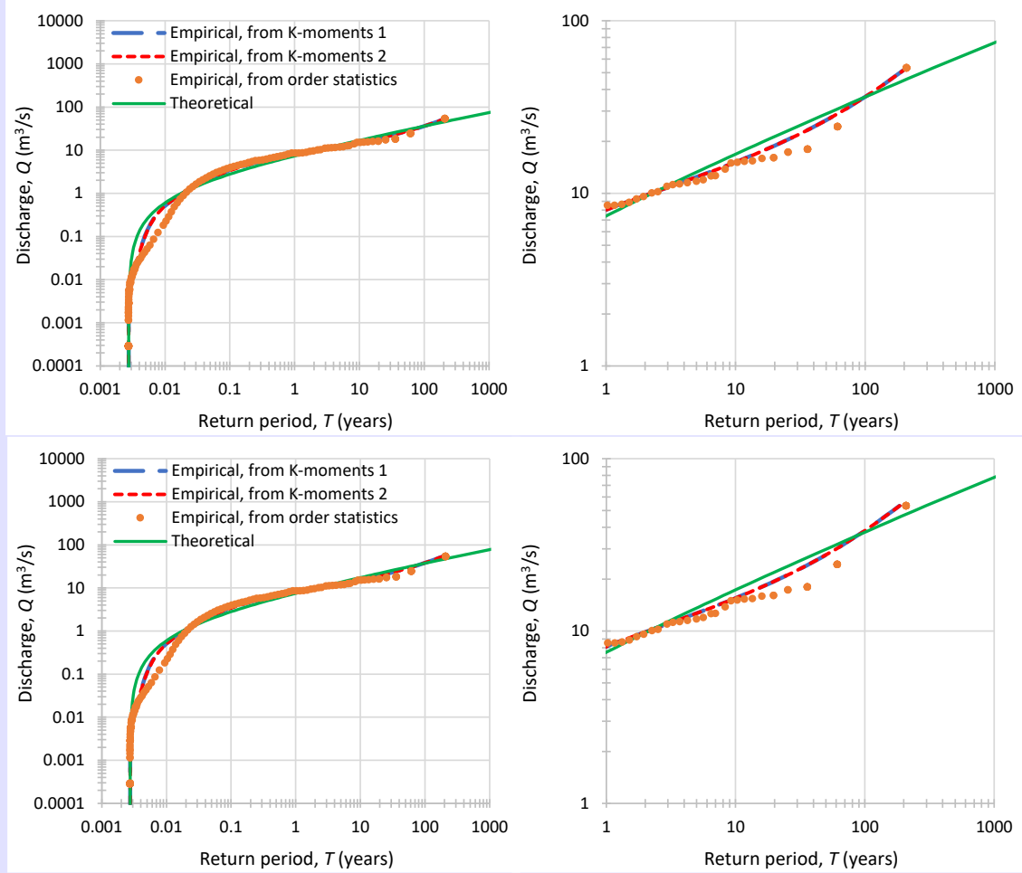
Figure 9.14 Comparison of empirical and theoretical (PBF) distributions fitted on daily data of the Tenmile Creek near Rimini, MT, USA, without ( upper ) and with ( lower ) bias adaptation (the points based on order statistics are not adapted in either case). The distribution function is depicted in terms of return period T , either over its entire range ( left column ) or focusing on values greater than 1 year ( right column ). The parameters are for the upper panels: \xi = 0.305, \zeta = 0.896, \lambda = 0.37 \text{ m}^3/\text{s}, x_L = 0 , and for the lower panels: \xi = 0.308, \zeta = 0.887, \lambda = 0.36 \text{ m}^3/\text{s}, x_L = 0 . For further explanations see caption of Figure 9.3.
