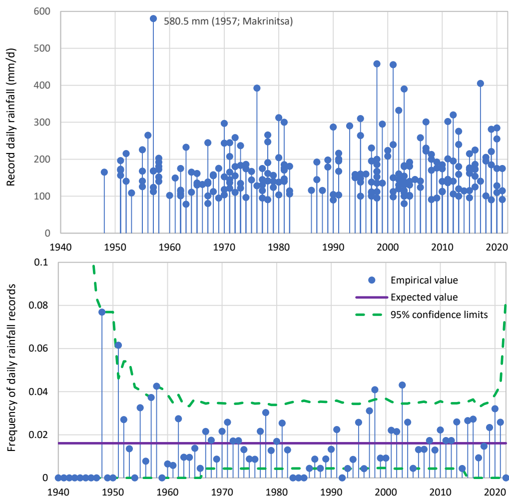
Figure 11.5 (upper) Records of maximum daily precipitation depth and (lower) frequency thereof per year for the 238 stations with long time series of annual maxima over the entire Greek territory. The confidence limits in the lower panel have been calculated from the binomial distribution, assuming independence and identical distribution. (Source: Koutsoyiannis et al., 2023b).
