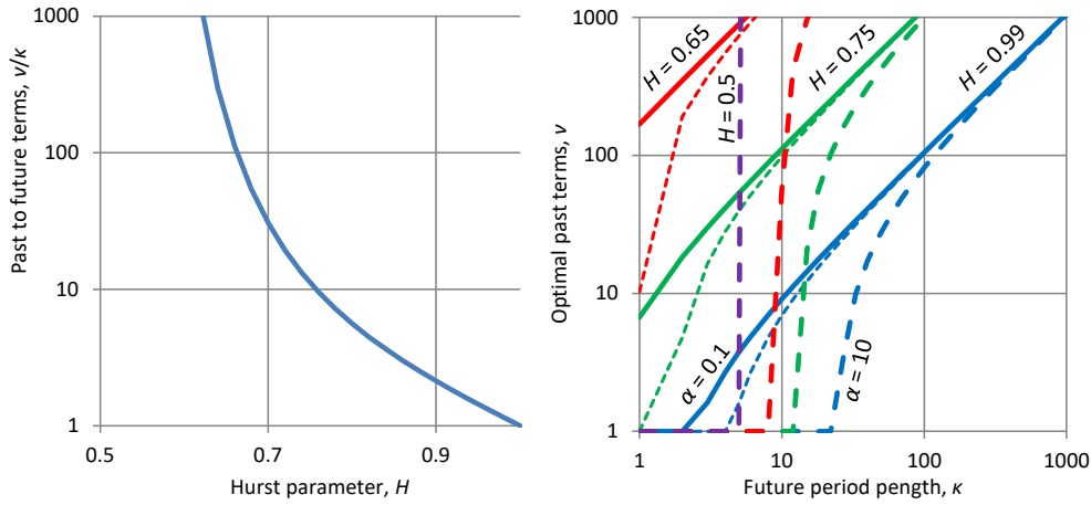
Figure 4.5 (left) Graphical illustration of equation (4.69) assuming a large length n of the time series. (right) Characteristic curves of optimal \nu vs \kappa for the indicated values of parameters H and \alpha as found by numerical analysis (and approximated by equation (4.72)); continuous, dotted and dashed lines correspond to \alpha = 0.1 , 1 and 10, respectively (for the case H = 0.5 the curves for \alpha = 0.1 and 1 fall out of the graph and therefore only that for \alpha = 10 is shown, which is a vertical straight line).
