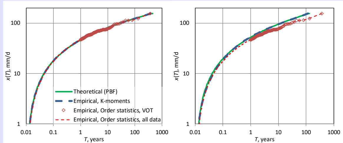
Figure 6.33 Same as Figure 6.32, but for the Pareto-Burr-Fuller distribution fitted for the entire range of return period, (left) assuming independence and (right) accounting for long-range dependence; note that empirical return periods based on order statistics do not consider dependence and thus they are the same in both panels.
