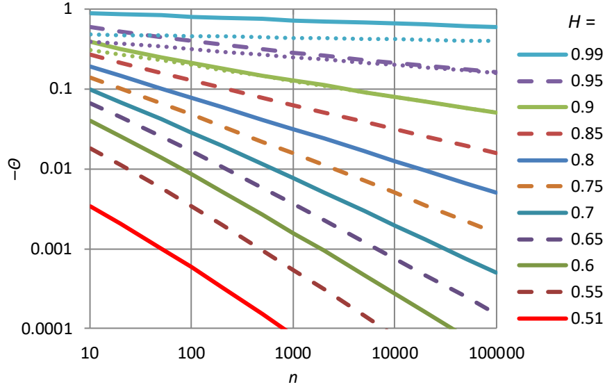
Figure 6.22 Adjustment coefficient \theta \left( \equiv \theta^{\text{HK}}(n, H) \right) of the upper central K-moment for q = 1 for a Hurst-Kolmogorov process with the indicated Hurst parameters. The results plotted are the first and second-order approximations, with the former plotted as dotted lines of the same colour as the latter, being indistinguishable from the latter, except for the three highest values of H (0.99, 0.95, 0.9), for which there are departures visible in the graph.
