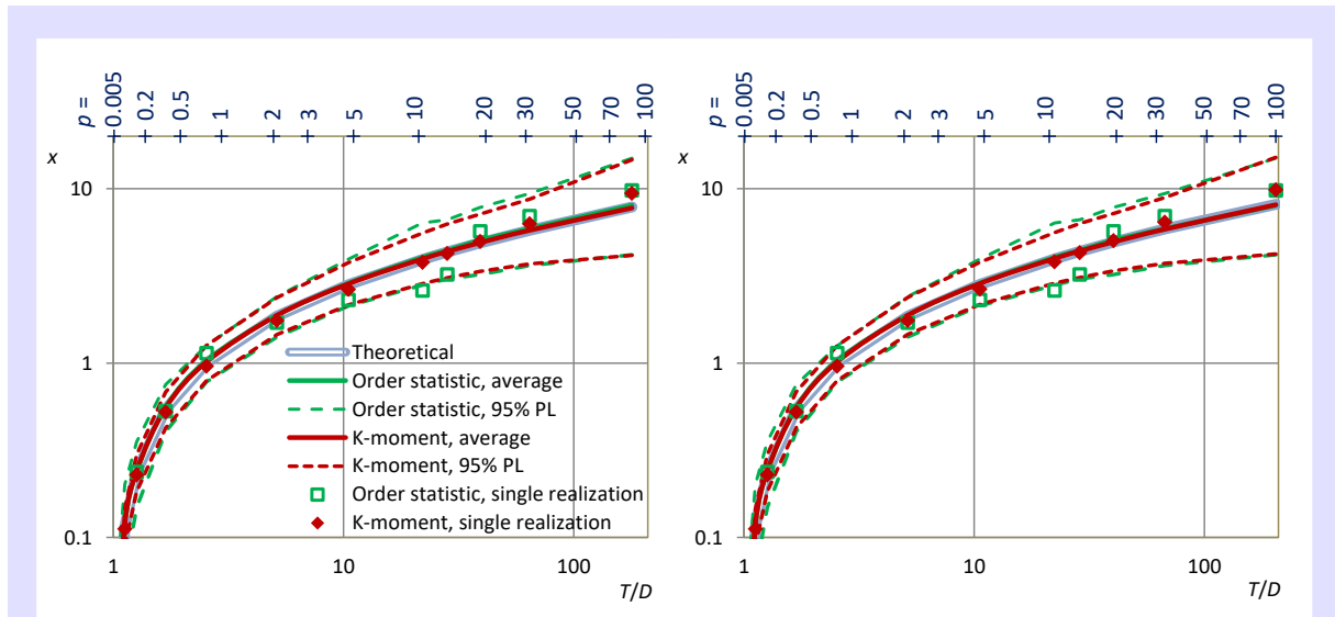
Figure 6.29 Simulation results of empirical return periods assigned to Pareto quantiles (for upper-tail index \xi = 0.15 , scale parameter \lambda = 1 and lower bound zero). Averages and prediction limits (PL) were calculated from 200 simulations each with n = 100 . The curves of averages for both the order statistics and the K-moment approaches are indistinguishable from the theoretical curves. The return periods T_{(i:n)} were assigned by (left) the generic option of unbiased \ln T and (right) the unbiased quantile option. The correspondence between the K-moment of order p and the return period T is also shown through the upper horizontal axis. The plots of a single realization are also shown (but only for part of the empirical points to avoid an overcrowded graph).
