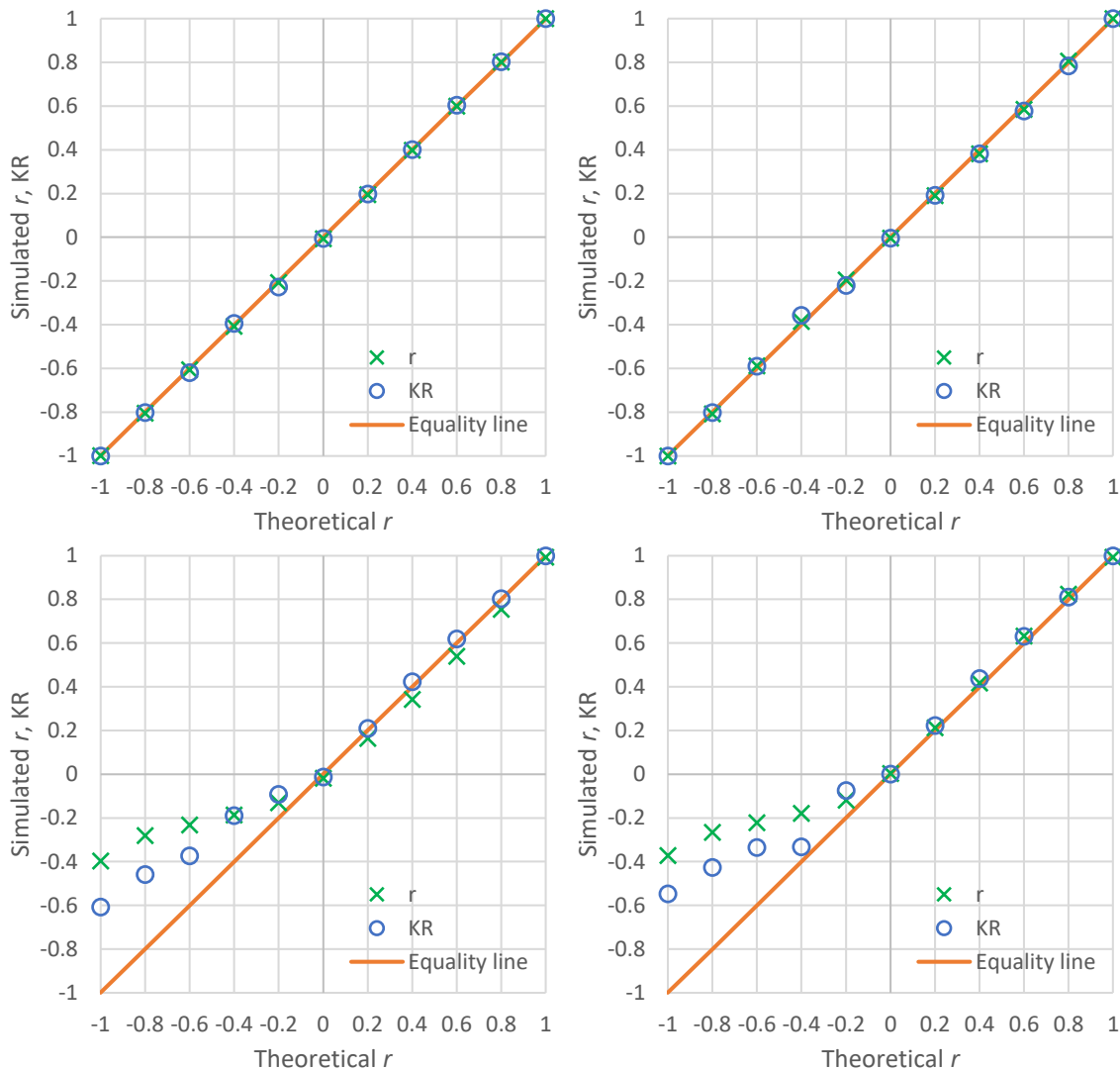
Figure 6.20 Simulation results of standard correlation ( r ) and K-correlation (KR) for a pair of stochastic variables nonlinearly dependent, obtained by 10 000 pairs generated by the method discussed in section 7.6, with identical marginal distribution, which for the four panels, seen clockwise, is: uniform, normal, lognormal with shape parameter \zeta = 1 , and Pareto with upper-tail index \xi = 0.25 .
