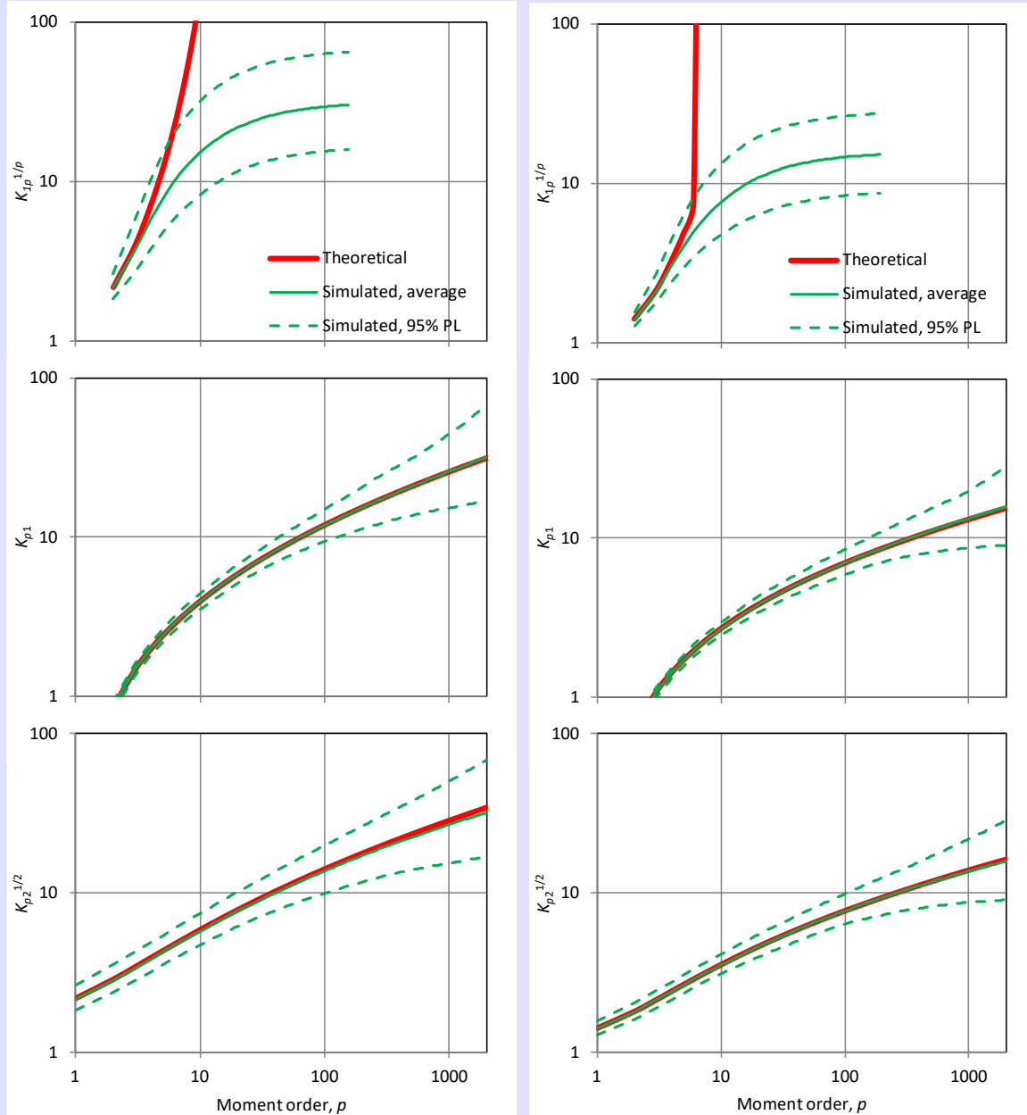
Figure 6.7 Illustration of the performance of the K-moment estimator of equations (6.60)–(6.62), applied to upper central K-moments, for the lognormal distribution ( left column ; \text{LN}(0,1) ) and the Pareto distribution ( right column ; upper-tail index \xi = 0.15 scale parameter \beta = 1 , lower bound zero) for q = 1 ( middle row ) and q = 2 ( bottom row ). For comparison, the performance of the estimators of classical moments is also shown ( upper row ; notice that in the Pareto distribution the true moments are \infty for p > 1/0.15 = 6.87 ). The true moments were determined by numerical integration for the lognormal distribution and from the equations in Table 6.2 for the Pareto distribution. The estimates are averages of 100 simulations each with n = 2000 and are indistinguishable from the true (theoretical) values. The 95% prediction limits (PL) are also shown.
