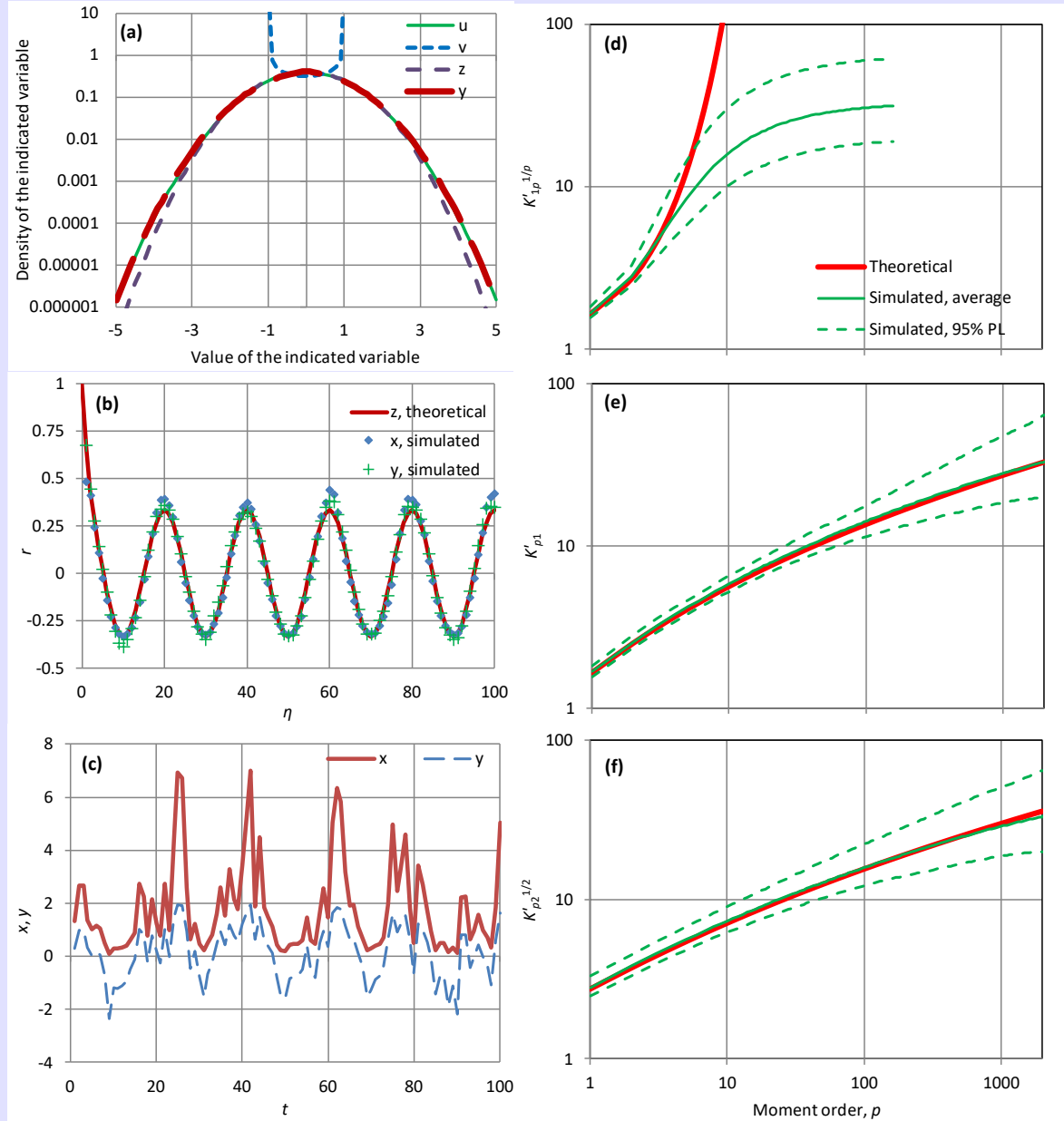
Figure 6.24 Illustration of theoretical and simulated results for the example in Digression 6.M, where the final process \underline{x} has lognormal marginal distribution \text{LN}(0,1) , the lag-1 autocorrelation of the Markov process is r = 0.5 and the period of the periodic component is a = 20 : (a) probability densities of variables \underline{u} , \underline{v} , \underline{z} and \underline{y} ; (b) autocorrelation of processes \underline{z} , \underline{x} and \underline{y} ; (c) 100 terms of time series from processes \underline{x} and \underline{y} ; (d) classical moments; (e)–(f) K-moments for q = 1 and 2 . Panels (d)–(f) are identical to those of Figure 6.7 (left), which is for the same marginal distribution. The estimates are averages of 100 simulations each with n = 2000 and in the case of K-moments are indistinguishable from the true (theoretical) values.
