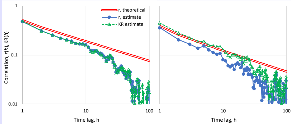
Figure 6.21 Empirical autocorrelation ( r ) and K-autocorrelation (KR) functions estimated from a simulated series with 10 000 values from an HK process with (left) normal and (right) lognormal distribution, also compared with the theoretical autocorrelation functions.
