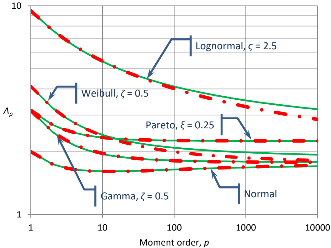
Figure 6.27 Illustration of the approximation of \Lambda -coefficients achieved by equation (6.161) for the indicated distribution functions.
