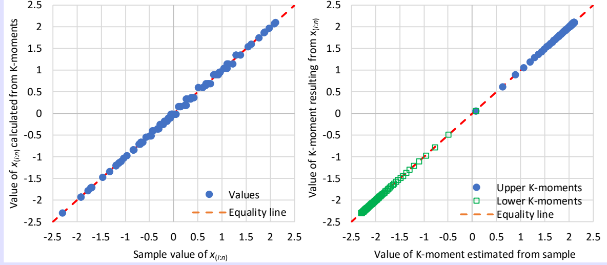
Figure 6.18 (left) Values of the order statistics calculated from K-moments by linear programming, vs. their true values. (right) K-moments re-determined from the calculated order statistics vs. the ones originally determined from the true order statistics.
