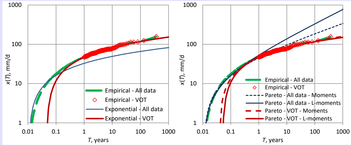
Figure 6.31 Fitting (in terms of plot of quantile x vs. return period T ) of the exponential ( left ) and Pareto ( right ) distribution on the Bologna daily rainfall record by the indicated methods; the empirical distribution is calculated by formula IV of Table 5.5.
