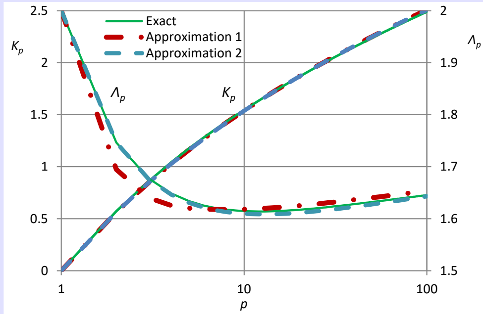
Figure 6.28 Comparison of approximate and exact values of K-moments and \Lambda -coefficients for the normal distribution. Approximations 1 and 2 are calculated by equations (6.169) and (6.171), respectively, and the exact values are calculated by numerical integration.
