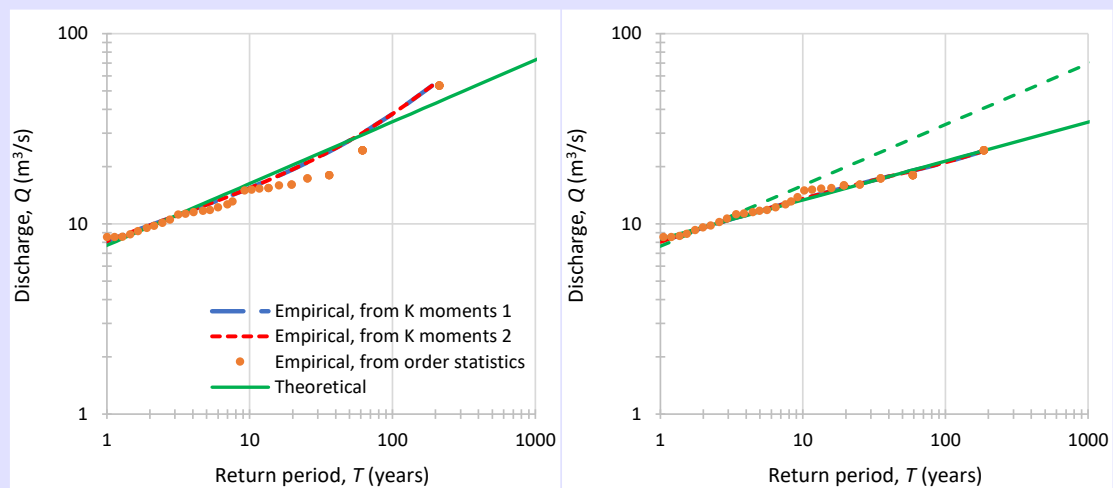
Figure 9.15 Comparison of empirical and theoretical (PBF) distributions fitted on daily data of the Tenmile Creek near Rimini, MT, USA, as in Figure 9.14 but with a fitting on T > 1 year by considering the highest value ( left ) or not ( right ). The fitted theoretical distribution of the left panel is also plotted on the right panel as dashed line. The parameters are, for the left panel: \xi = 0.325, \zeta = 5.08, \lambda = 1.25 \text{ m}^3/\text{s}, x_L = 0 , and for the right panel: \xi = 0.205, \zeta = 20, \lambda = 2.67 \text{ m}^3/\text{s}, x_L = 0 .
