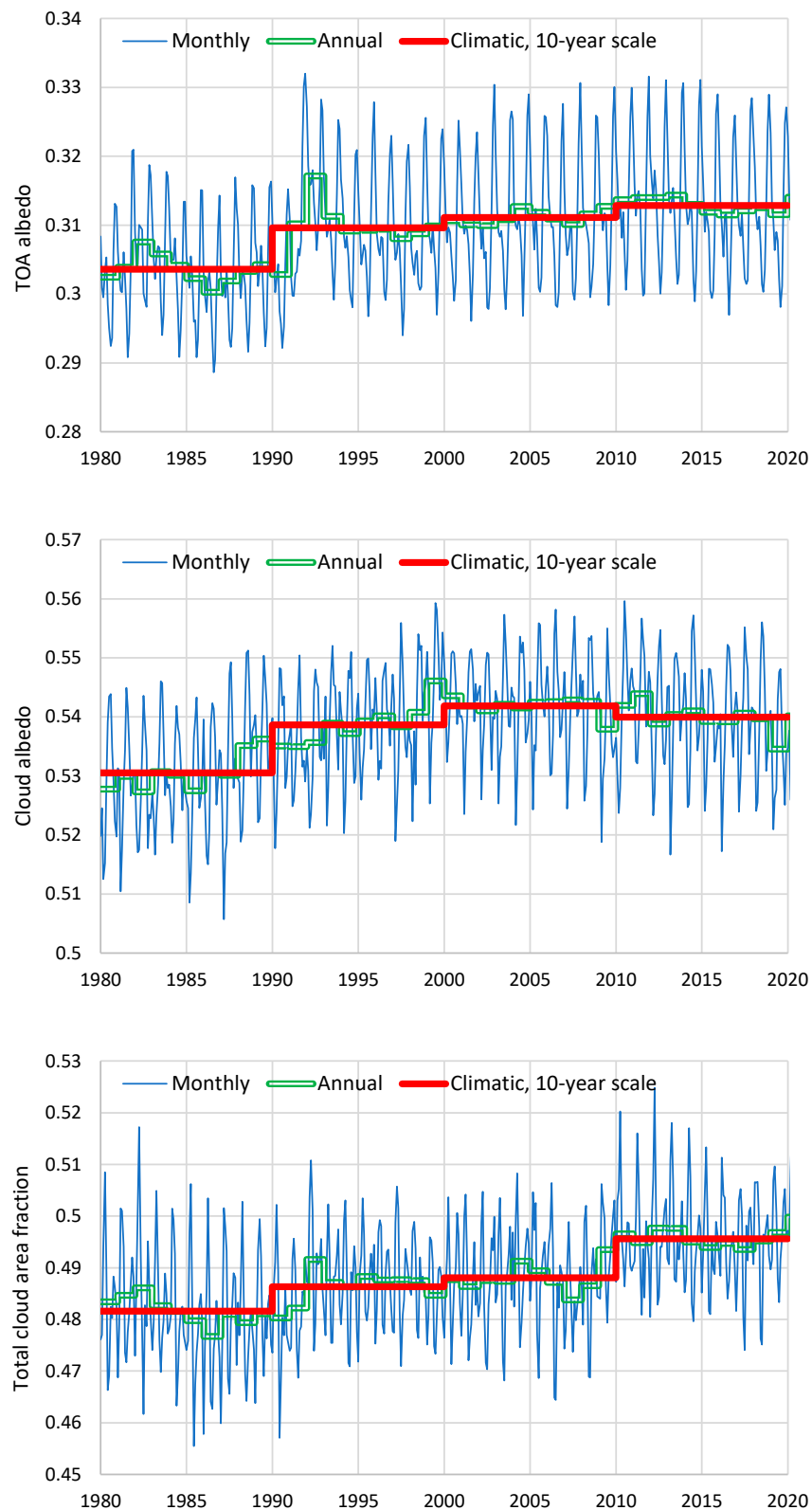
Figure A4. Time series of ( upper ) TOA albedo, ( middle ) cloud albedo and ( lower ) total cloud area fraction, as provided by NASA's MERRA-2 International Satellite Cloud Climatology Project (ISCCP).
