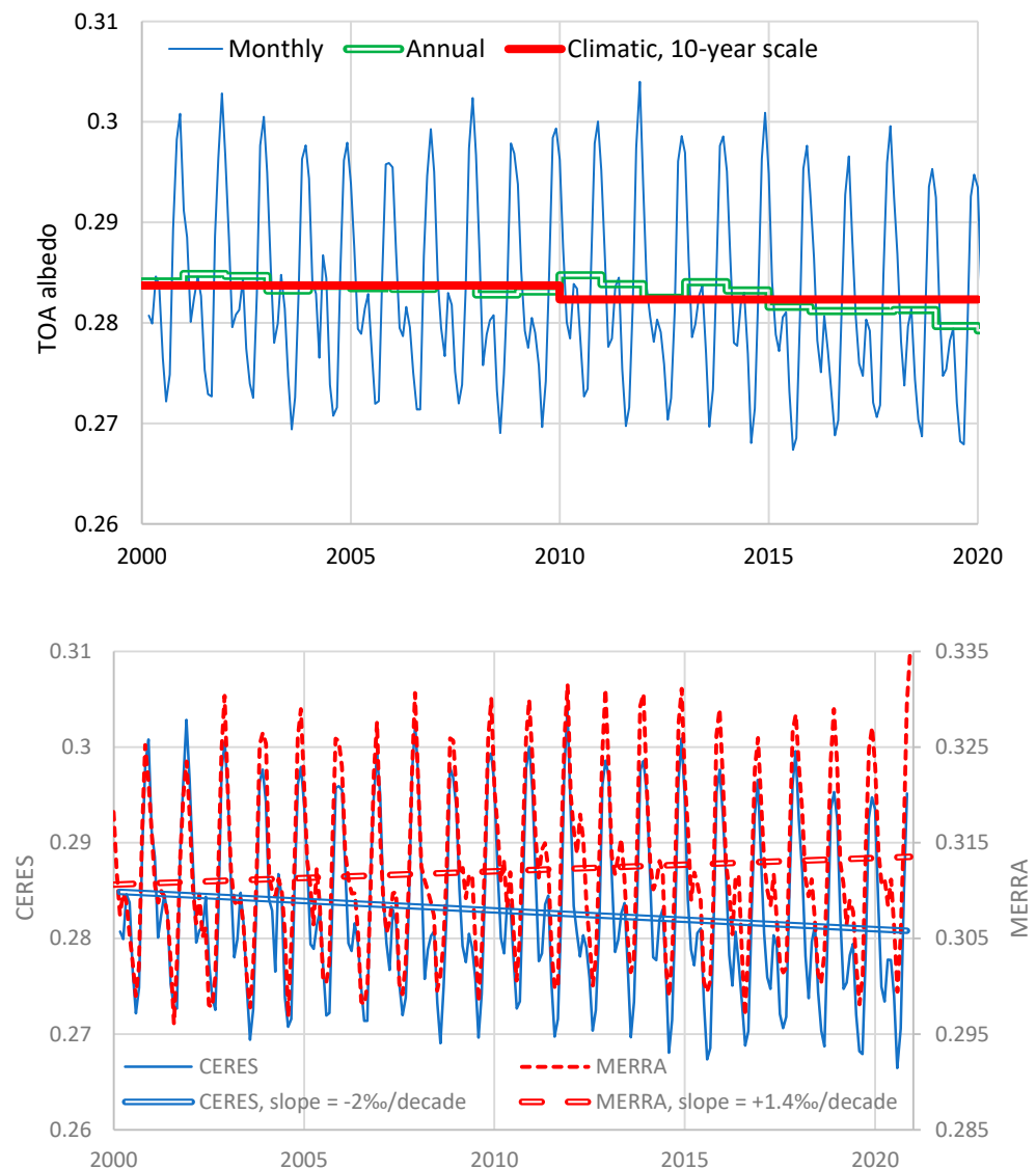
Figure A5. (Upper) TOA albedo time series, as provided by NASA’s Clouds and the Earth’s Radiant Energy System (CERES); (lower) the same series on annual time scale in comparison of the MERRA-2 series (Figure A4, upper panel) along with linear trends plotted for both series with fitted slopes shown in the legend.
