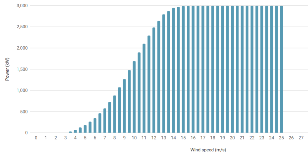
Power curve
