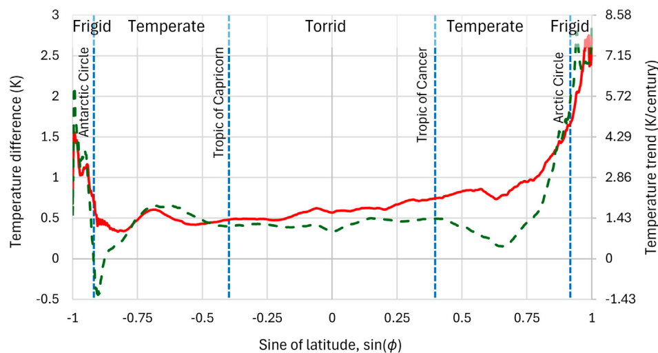
FIGURE 14 Difference of average surface temperatures, as a function of the sine of latitude, of two 30-year climatic periods, namely, of the most recent 1995 – 2024 minus the 1950 – 1979. Continuous line represents the average over the globe, while dashed line represents the average over the area between longitudes 155°E and 130°W, mostly covered by sea (Pacific, Arctic and Southern Oceans). The sine of latitude was chosen as the horizontal axis so that increments be proportional to the respective areas on Earth. Data from ERA5 reanalysis; data retrieval and processing from the CLIMEXP platform (processing steps: (a) subsetting for each of the two periods; (b) aggregation to annual (Jan-Dec) time resolution; (c) compute zonal mean; (d) compute mean, s.d. [standard deviation], or extremes).
