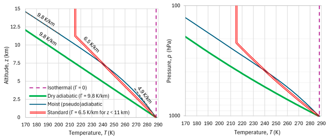
FIGURE 6 Comparison of different models of temperature profiles of Earth's troposphere, in terms of (left) altitude and (right) pressure (in logarithmic axis).
