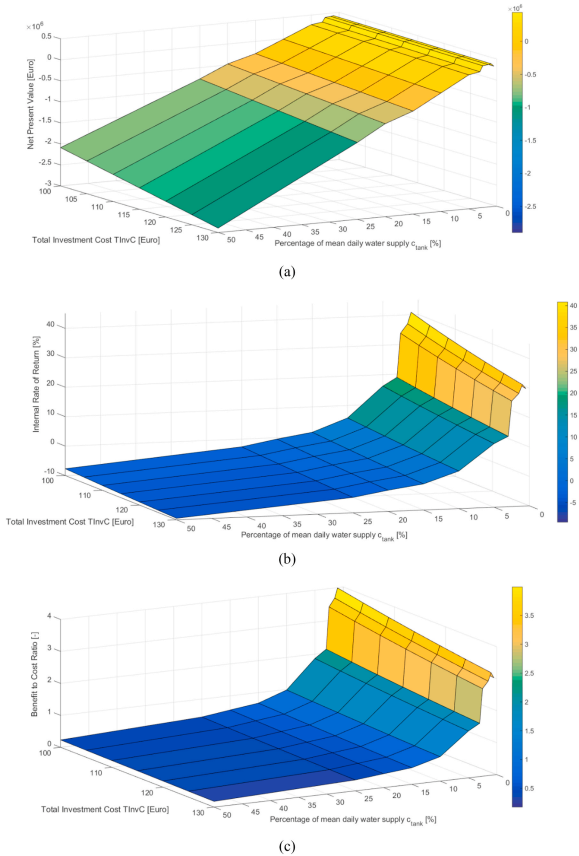
Fig. 10. (a) Net Present Value, (b) Internal Rate of Return, (c) Benefit to Cost ratio for the eleven examined scenarios of tanks with different percentage of mean daily water supply, for different Total Investment cost (100 %–130 % of base value).
