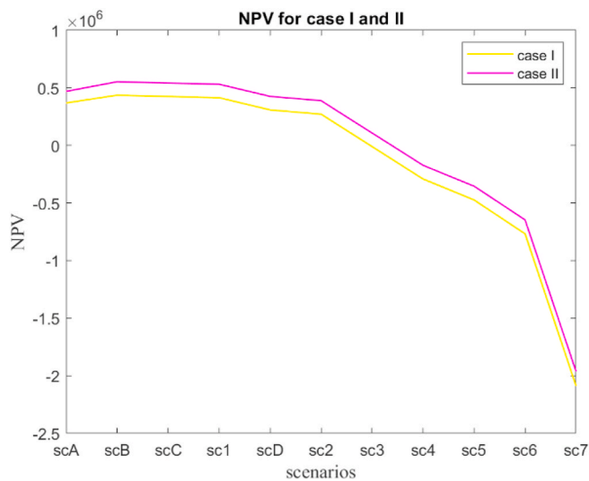
Fig. 6. Net Present Value for the eleven examined scenarios, for two cases of energy cost (I: net cost of electricity 0.097 \text{ €/kWh} , II: net cost of electricity 0.116 \text{ €/kWh} ).
