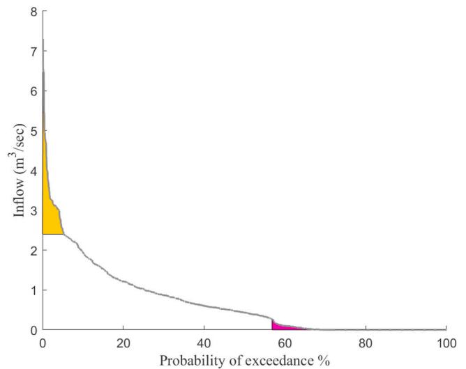
Fig. 1. Flow duration curve and volumes of unexploited areas due to lack of storage in SHPPs.
