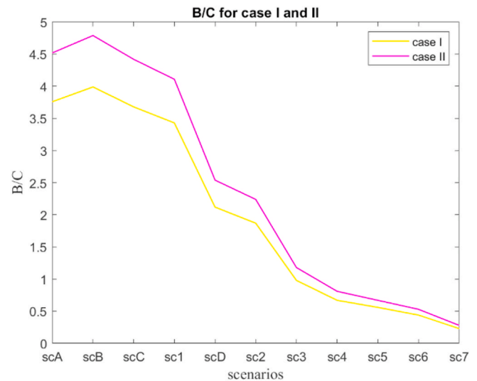
Fig. 8. Benefit to Cost ratio for the eleven examined scenarios, for two cases of energy cost (I: net cost of electricity 0.097 \text{ €/kWh} , II: net cost of electricity 0.116 \text{ €/kWh} ).
