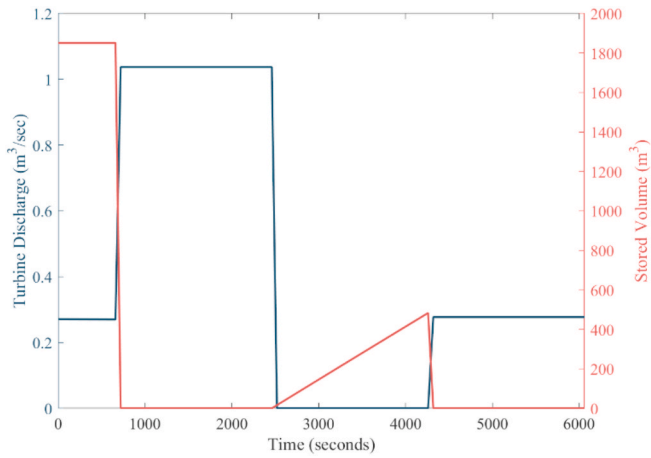
Fig. 5. Results of turbine's simulated operation, in terms of exploited discharge, on May 31, 2018 for scenario Sc_D .
