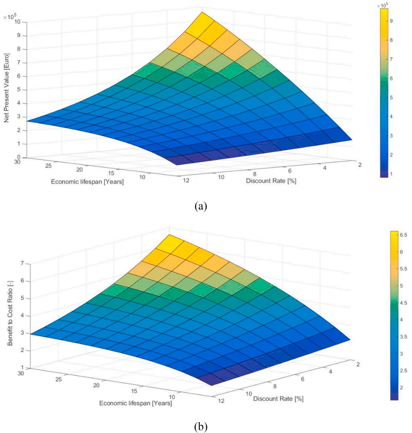
Fig. 14. (a) Net Present Value, (b) Benefit to Cost ratio for the scenario Sc_B (tank of a 1 % of the mean daily water supply) for different economic lifespan (6–30 years) and different discount rate (2 %–12 %).
