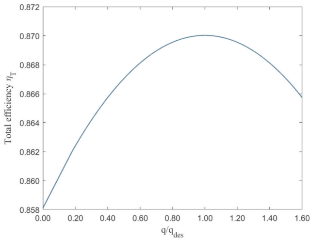
Fig. 4. Approximated total efficiency curve with respect to q/q_{des} ratio.
