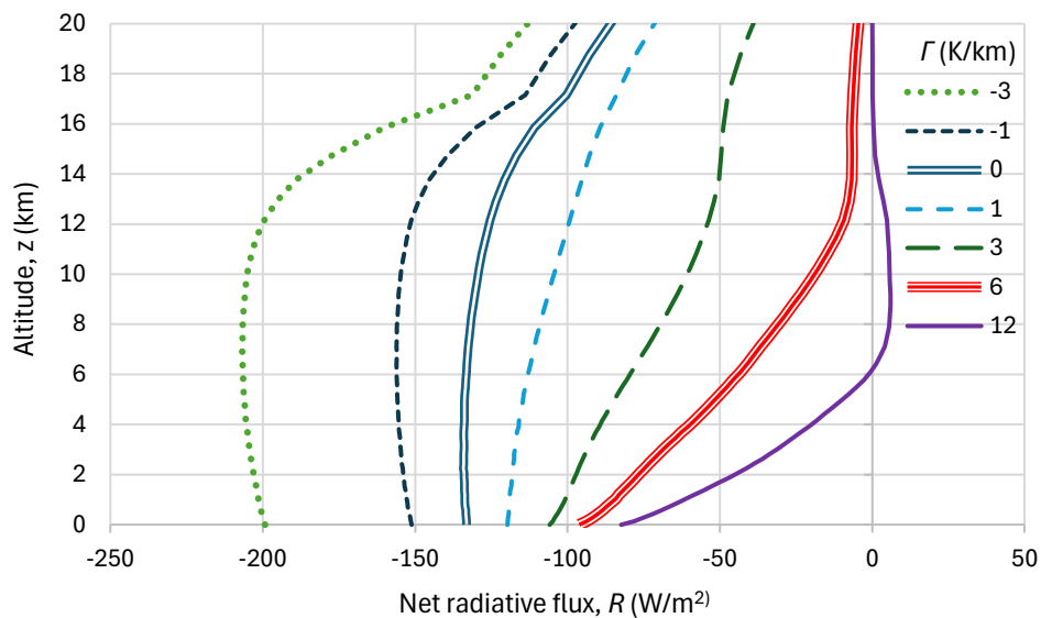
Figure 7.19 Vertical distribution of net radiation flux for the RRTM runs of Figure 7.17, for different lapse rates.
