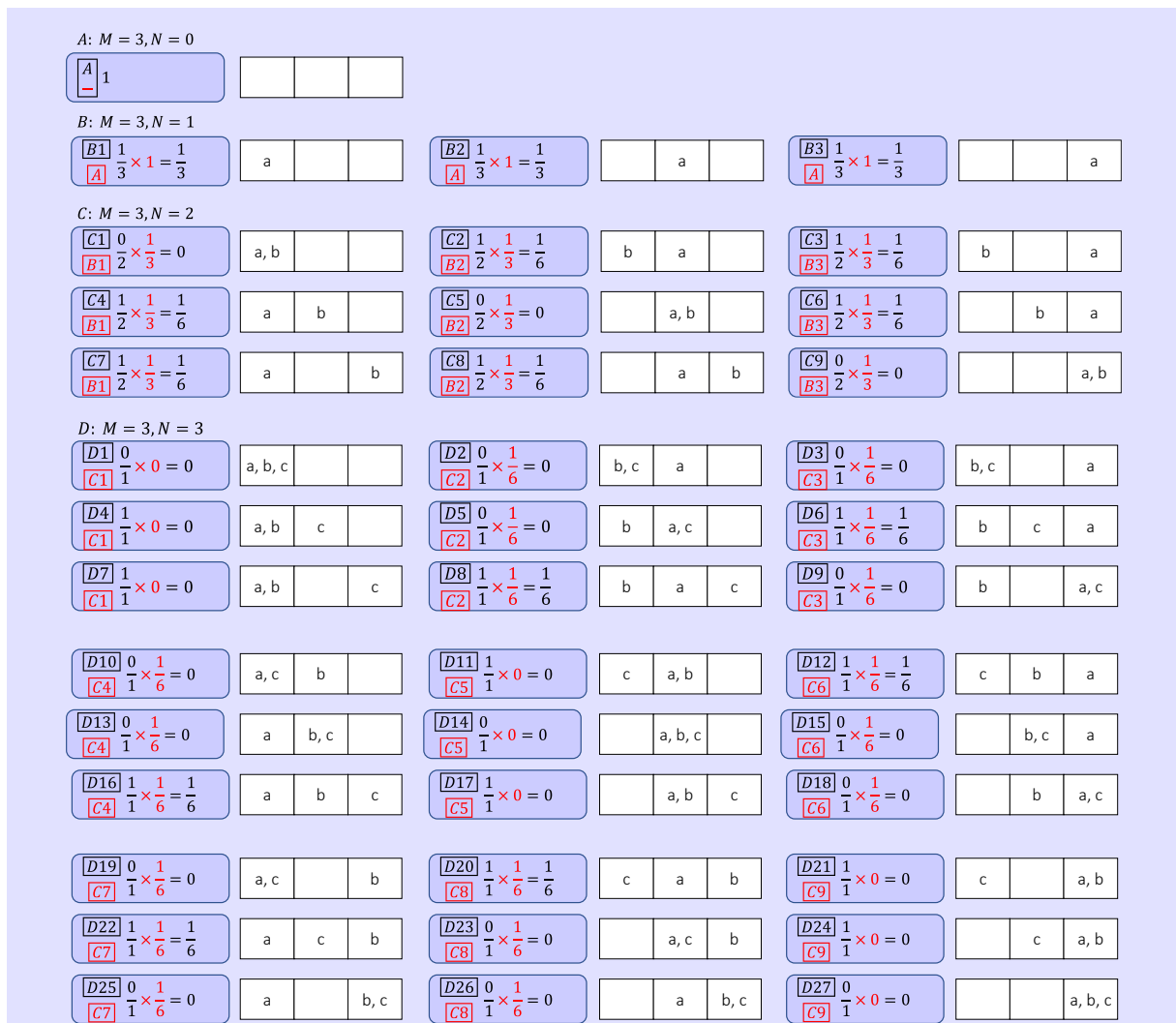
Figure 5.4 Illustration of calculating probabilities of all possible arrangements by putting up to N = 3 negatively dependent distinguishable particles (fermions), designated as a, b, c, into M = 3 boxes. Each arrangement is given a particular label (B1, B2, etc.; upper in each container of calculations) accompanied with the label of the predecessor arrangement (lower left in each container of the calculations). In each calculation the first term is the conditional probability according to equation (5.17) and the second term is the probability that the condition holds, as calculated in the predecessor arrangement (i.e. the calculation is: conditional probability \times predecessor probability equals probability of this arrangement).
