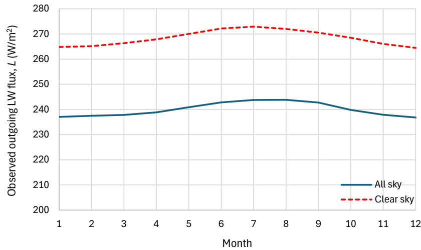
Figure 7.12 Monthly variation of outgoing LW radiation flux for 2024. The annual average is 240 and 268 \text{W/m}^2 for all sky and clear sky, respectively. Data from NASA's CERES site for Terra platform (Edition 4.2; https://ceres-tool.larc.nasa.gov/ord-tool/jsp/SSF1degEd42Selection.jsp ).
