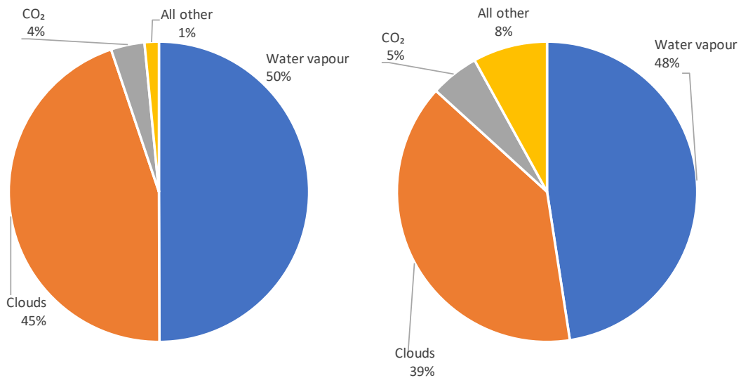
Figure 7.25 Contribution of the ARE drivers to the LW radiation fluxes, ( left ) downwelling and ( right ) outgoing. (Source: Koutsoyiannis, 2024.)
