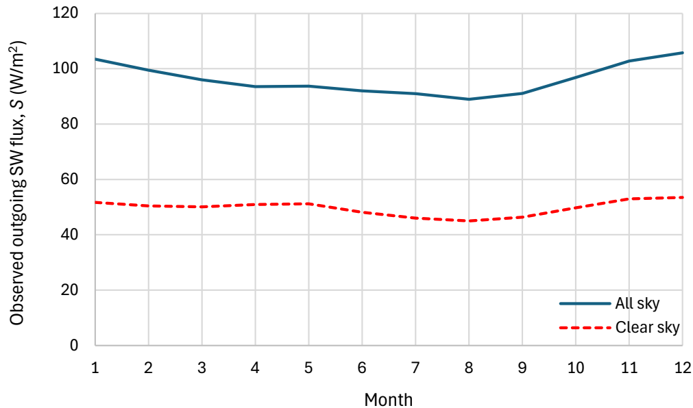
Figure 7.10 Monthly variation of outgoing solar radiation flux for 2024. The annual average is 96.2 and 49.7 W/m 2 for all sky and clear sky, respectively. Data from NASA’s CERES site for Terra platform (Edition 4.2; https://ceres-tool.larc.nasa.gov/ord-tool/jsp/SSF1degEd42Selection.jsp ).
