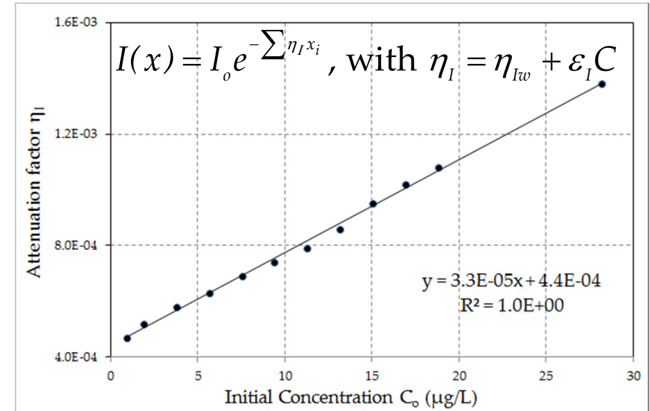
Figure 2: Light intensity attenuation factors (slope and intercept of the trend-line). Where C is the R6G concentration and x_i the distance the laser beam travels through the water-tank (from pixel i to i-1 ).
