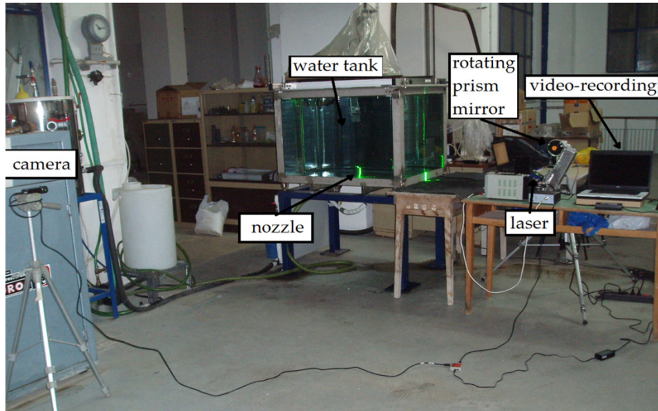
Figure 1: PLIF experimental set-up (NTUA, Laboratory of Hydraulics). The camera (for video tapping), nozzle, water-tank, rotating prism mirror, laser and video-recording (for video digitization) are shown.
