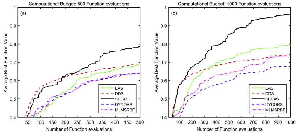
Fig. 12. Convergence curves for MFE = 500 (a) and MFE = 1000 (b).
