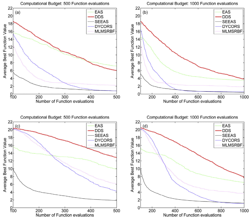
Fig. 4. Convergence curves for test function OF2 (Ackley) with 15 (a, b) and 30 variables (c, d), with MFE = 500 (a, c) and MFE = 1000 (b, d).
