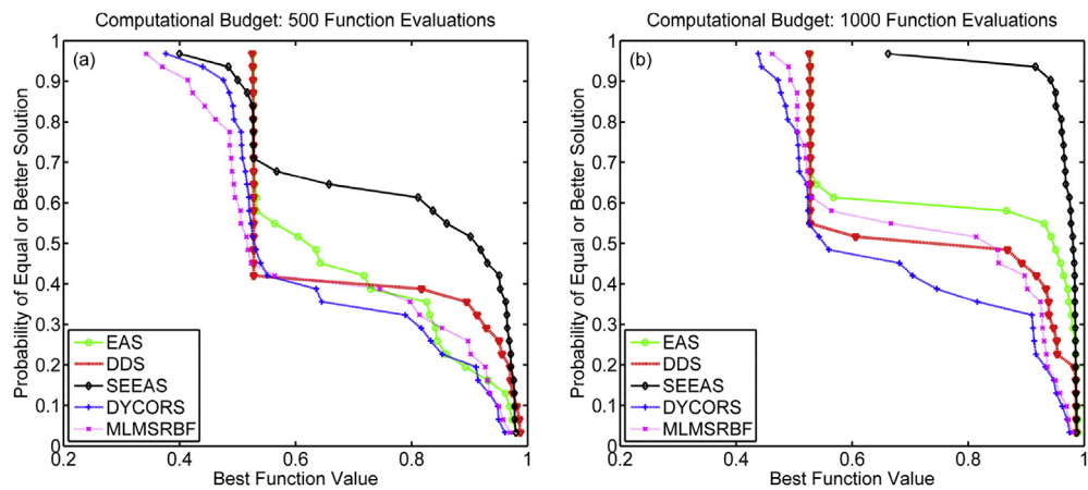
Fig. 13. Empirical CDFs of best NSE values for MFE = 500 (a) and MFE = 1000 (b).
