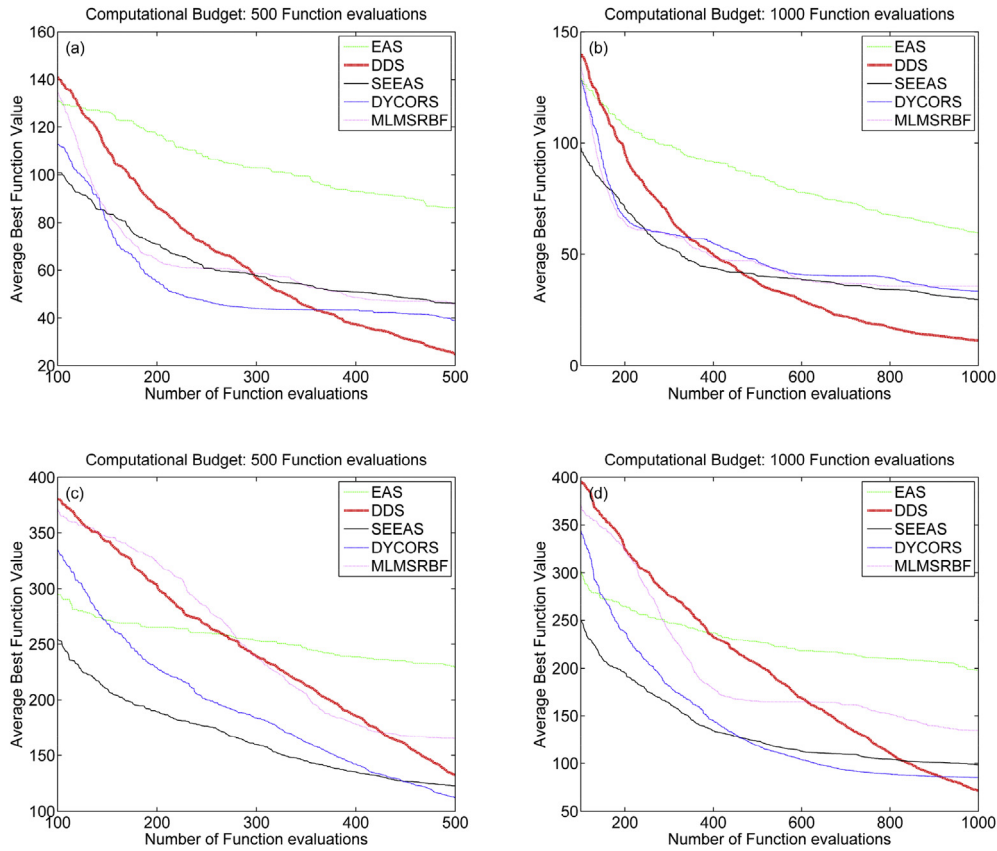
Fig. 7. Convergence curves for test function OF5 (Rastrigin) with 15 (a, b) and 30 variables (c, d), with MFE = 500 (a, c) and MFE = 1000 (b, d).
