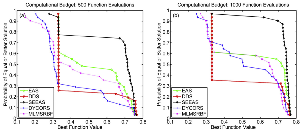
Fig. 11. Empirical CDFs of best NSE values for MFE = 500 (a) and MFE = 1000 (b).
