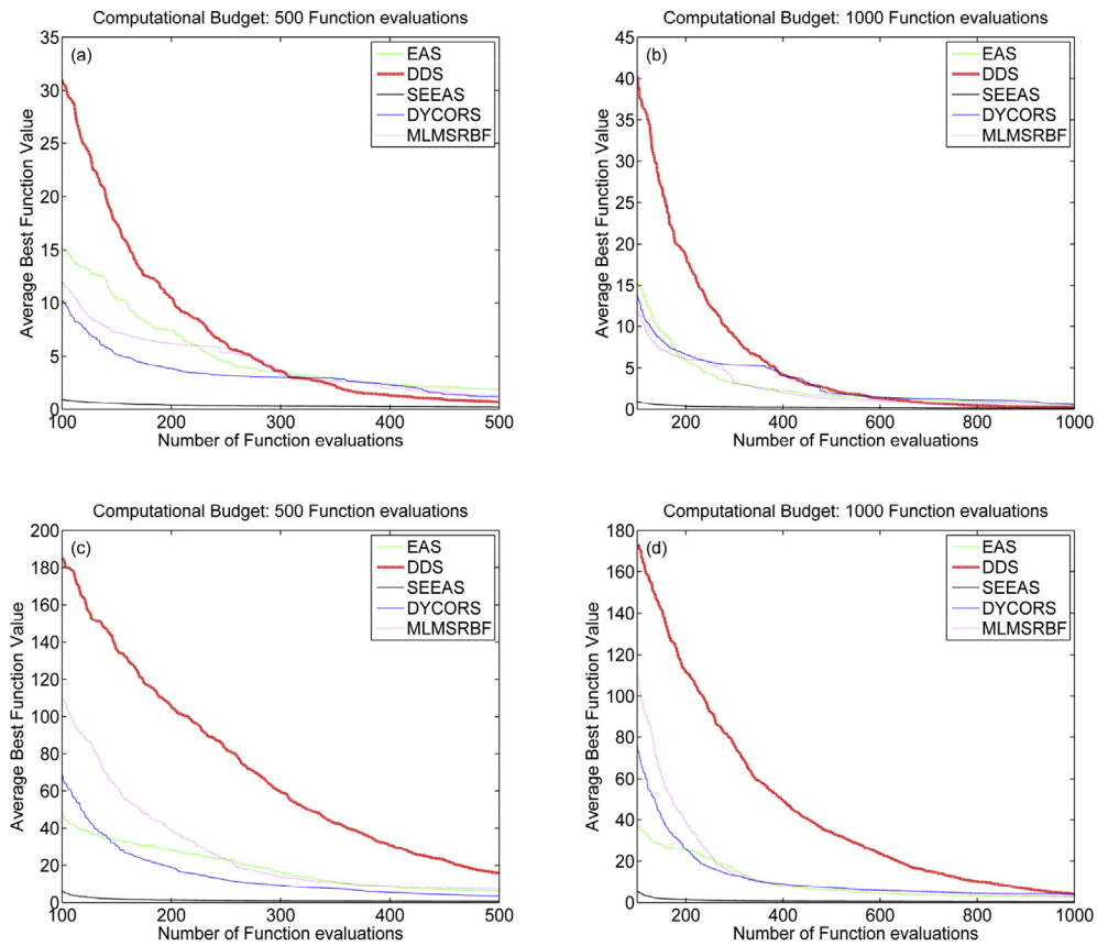
Fig. 8. Convergence curves for test function OF6 (Levy) with 15 (a, b) and 30 variables (c, d), with MFE = 500 (a, c) and MFE = 1000 (b, d).
