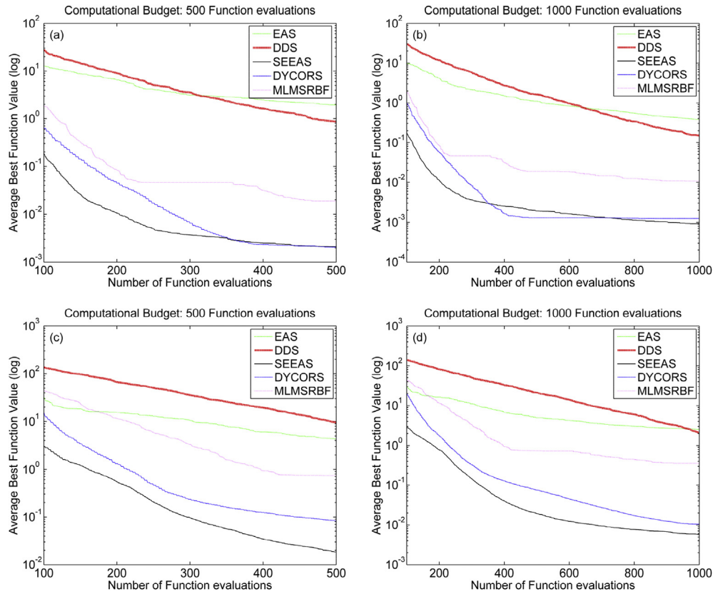
Fig. 3. Convergence curves for test function OF1 (Sphere) with 15 (a, b) and 30 variables (c, d), with MFE = 500 (a, c) and MFE = 1000 (b, d).
