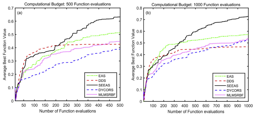
Fig. 10. Convergence curves for MFE = 500 (a) and MFE = 1000 (b).
