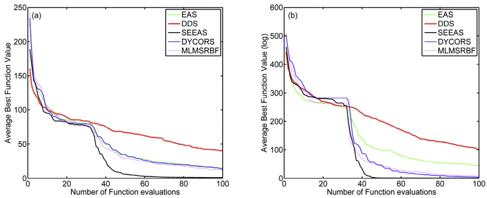
Fig. 9. Initial part of convergence curves up to 100 function evaluations, for test functions Levy (a) and Griewank (b), for the case of MFE = 500 and 15 variables.
