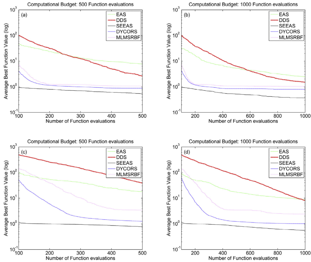
Fig. 5. Convergence curves for test function OF3 (Griewank) with 15 (a, b) and 30 variables (c, d), with MFE = 500 (a, c) and MFE = 1000 (b, d).
