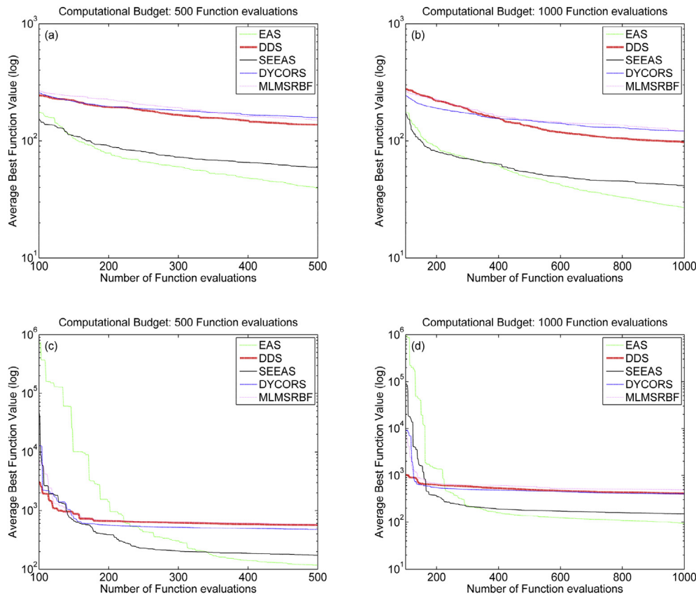
Fig. 6. Convergence curves for test function OF4 (Zakharov) with 15 (a, b) and 30 variables (c, d), with MFE = 500 (a, c) and MFE = 1000 (b, d).
