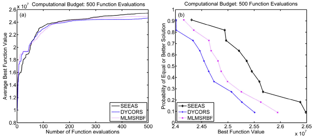
Fig. 14. Convergence curves (a) and empirical CDFs (b) for MFE = 500.
