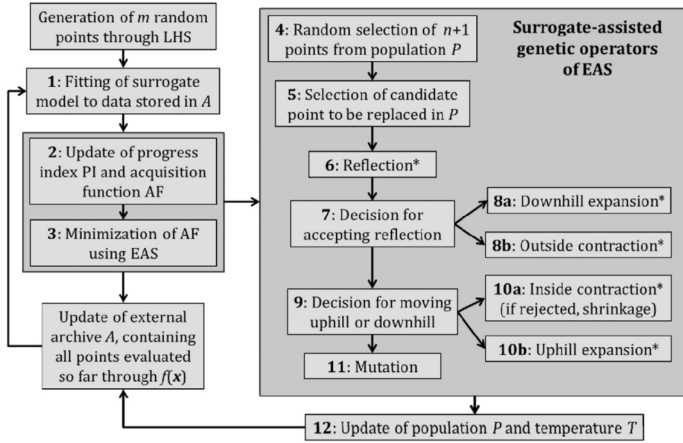
Fig. 2. Outline of SEEAS algorithm following the steps explained in Section 2.2.4 (* denotes the use of the surrogate model within the associated simplex transformations).
