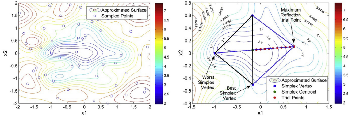
Fig. 1. Approximated surface (RBF) in a 2-D example (Ackley function) using all available sample points (left panel). The right panel demonstrates a randomly selected simplex and the modified surrogate-enhanced reflection movement using candidate points on the line formed from the simplex centroid and the maximum reflection point. The simplex is reflected at the candidate point with the minimum function value.
