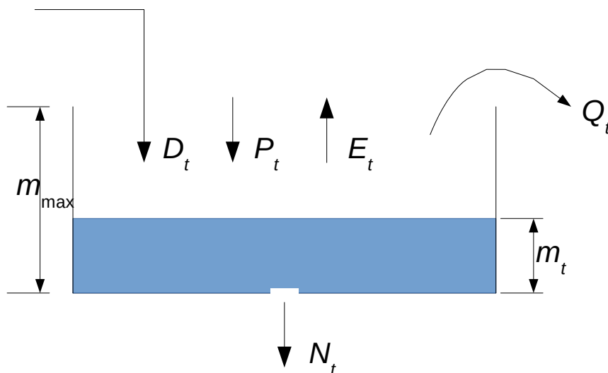
Figure 1. Soil moisture model used in UWOT to estimate latent heat and water demand.
