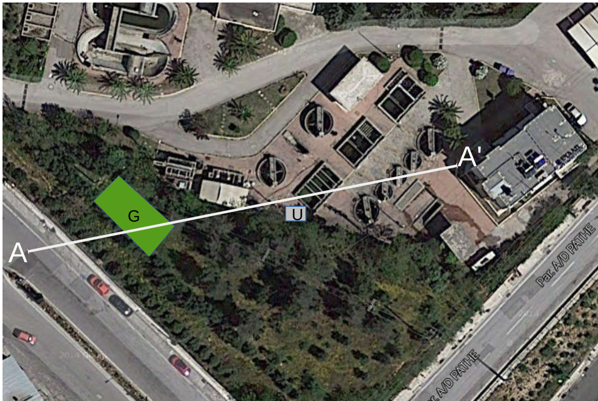
Figure 3. The irrigated green area (marked with the green rectangle G) and the compact treatment
