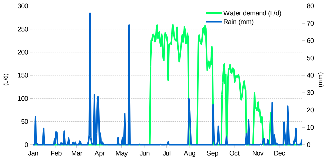
Figure 6. Water required during 1999 (as estimated by UWOT) for irrigating the 50 m 2 green area of the case study and rainfall depth during the same period.
