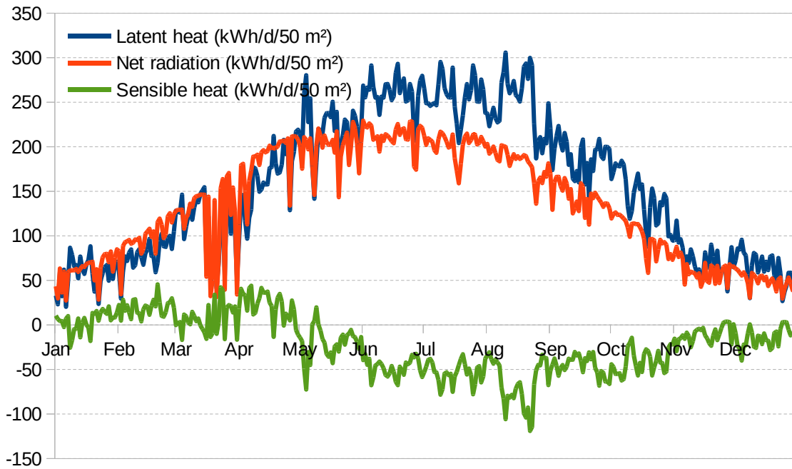
Figure 5. Heat fluxes over the 50 m 2 green area of the case study estimated by the UWOT simulation from 1 Jan 1999 to 31 Dec 1999.
