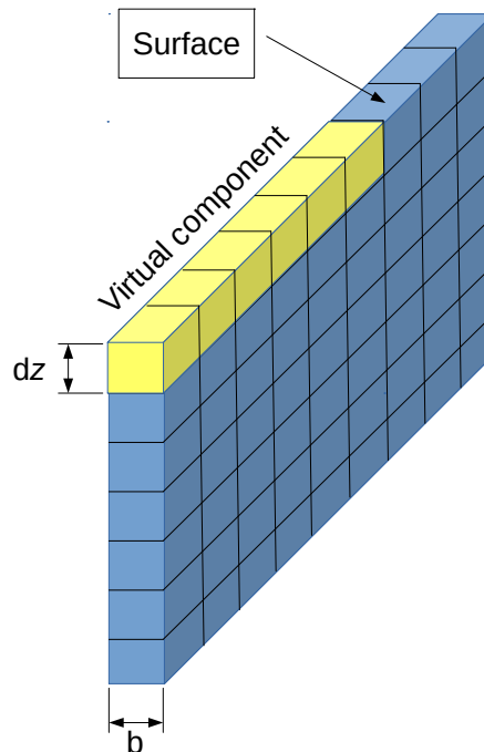
Figure 2. Part of the Energy2D grid (up to the land surface) with the virtual component highlighted.
