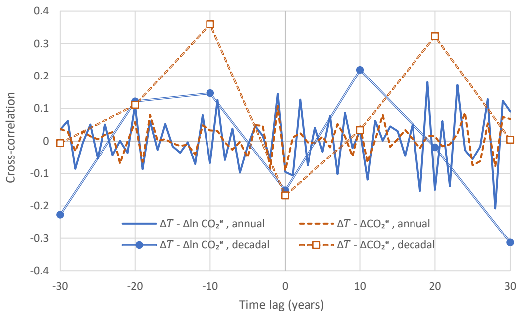
Figure SI5 Empirical cross-correlation function between the time series of differenced temperature at Central England, and global human \text{CO}_2^e , as well as logarithms of \text{CO}_2^e , at the annual and the 10-year time scale.
