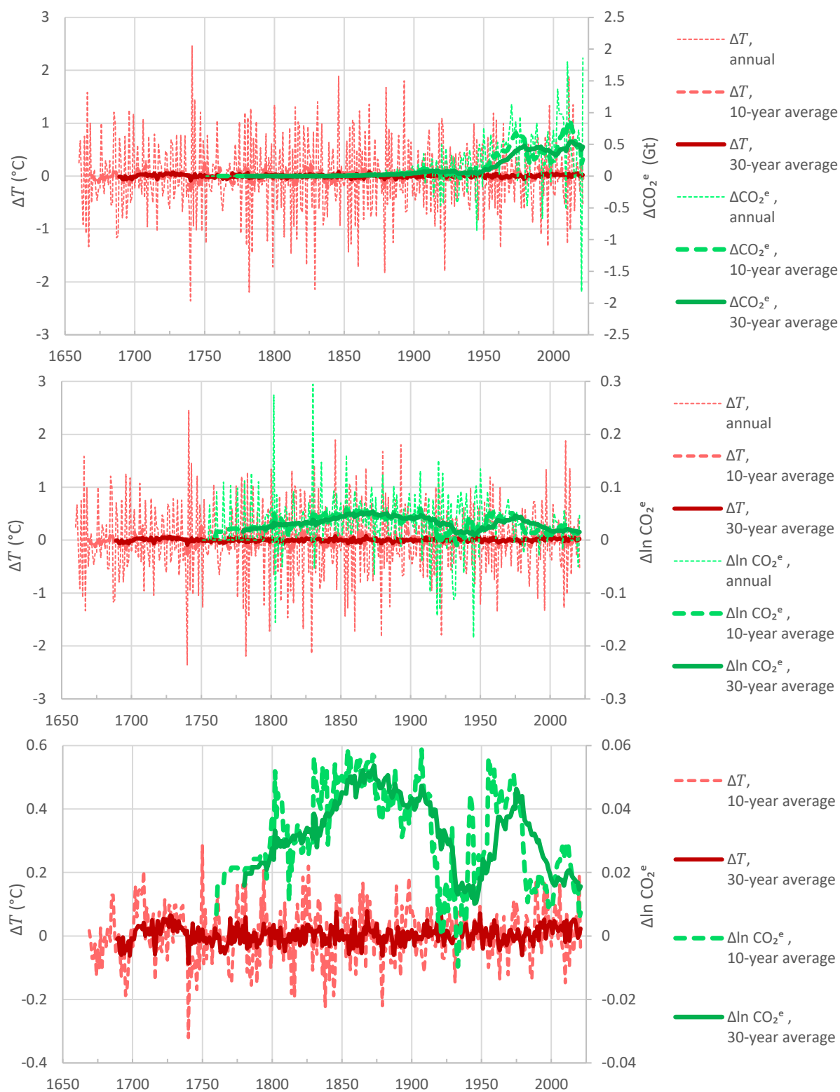
Figure SI4 Comparative evolution of the differenced time series of temperature at Central England, and the global human \text{CO}_2 emissions ( \text{CO}_2^e ) ( upper ), as well as logarithms of \text{CO}_2^e ( middle ). The 10- and 30-year averages are also plotted, in addition to annual values or without them ( lower ) to improve legibility.
