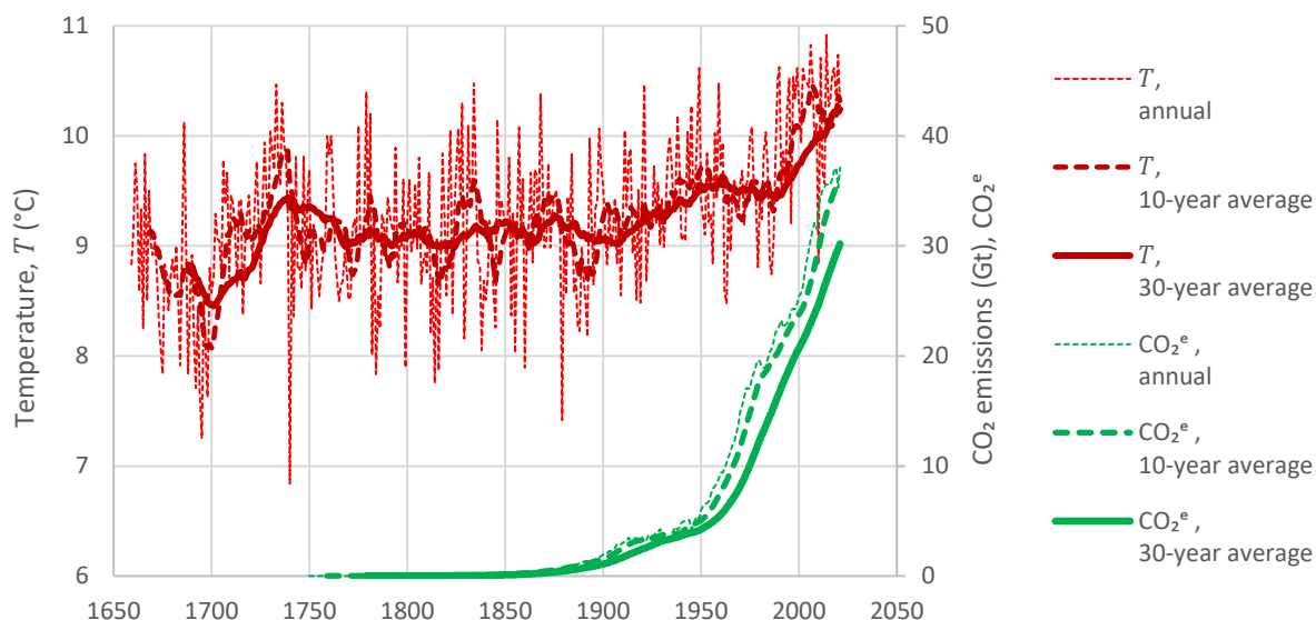
Figure SI3 Comparative evolution of global human CO 2 emissions (CO 2 e ) and temperature at Central England.
