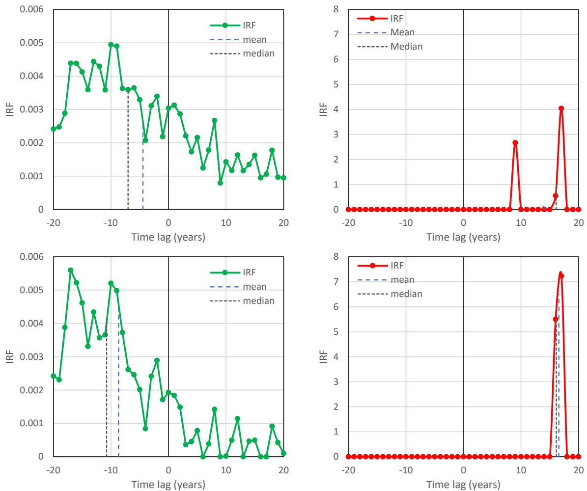
Figure S11 IRFs for temperature–CO 2 concentration based on the UKESM1-0 temperature and SSP2-4.5 CO 2 time series, respectively, calculated without using the roughness constraint; upper row : period 1850-2100—case studies #34 ( left ; \Delta T \rightarrow \Delta \ln[\text{CO}_2] ) and #35 ( right ; \Delta \ln[\text{CO}_2] \rightarrow \Delta T ); lower row : period 1850-2021—case studies #36 ( left ; \Delta T \rightarrow \Delta \ln[\text{CO}_2] ) and #37 ( right ; \Delta \ln[\text{CO}_2] \rightarrow \Delta T ).
