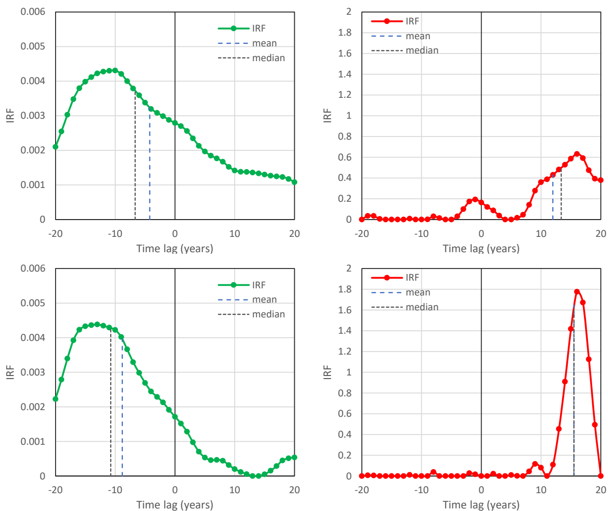
Figure SI2 IRFs for temperature–CO 2 concentration based on the UKESM1-0 temperature and SSP2-4.5 CO 2 time series, respectively, as in Figure SI1 but calculated using the roughness constraint; upper row : period 1850-2100—case studies #38 ( left ; \Delta T \rightarrow \Delta \ln[\text{CO}_2] ) and #39 ( right ; \Delta \ln[\text{CO}_2] \rightarrow \Delta T ); lower row : period 1850-2021—case studies #40 ( left ; \Delta T \rightarrow \Delta \ln[\text{CO}_2] ) and #41 ( right ; \Delta \ln[\text{CO}_2] \rightarrow \Delta T ).
