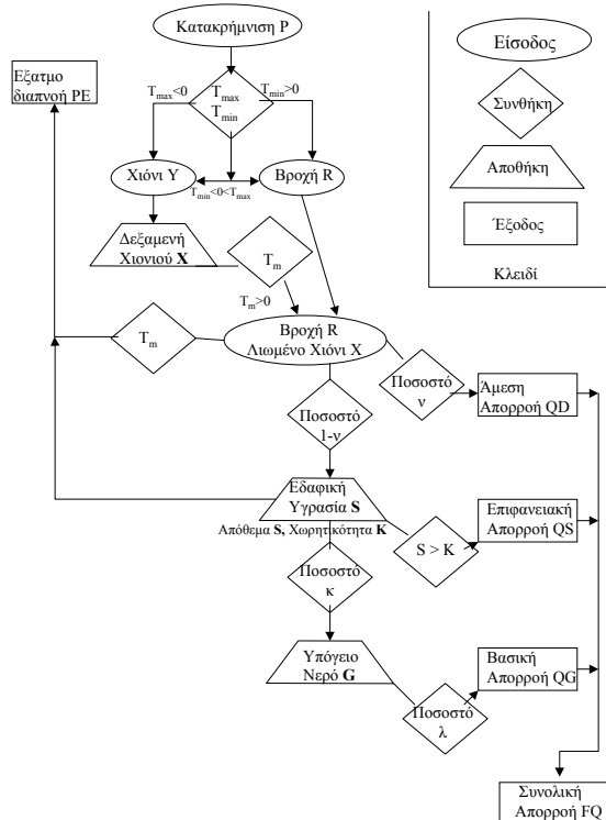
Figure 3: Flowchart of the model
