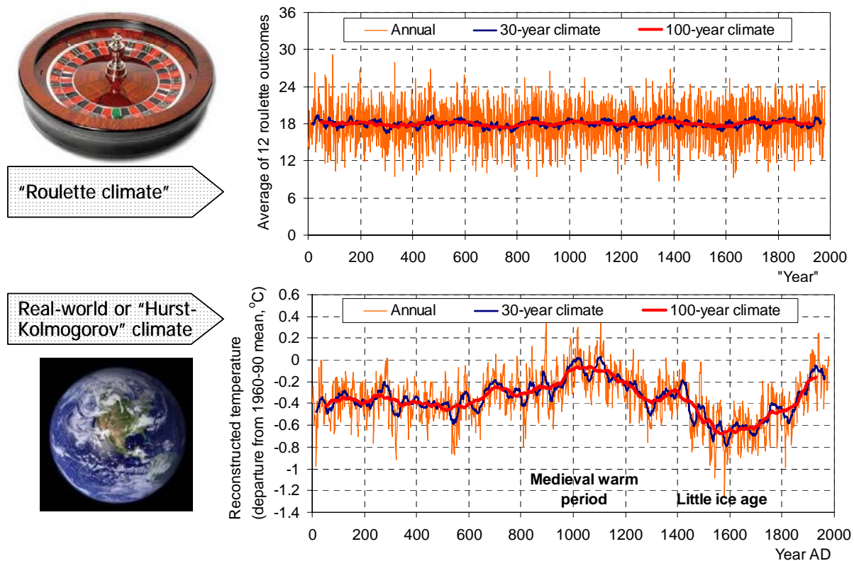
Figure 7: Demonstration of the differences between the classical statistical paradigm, represented by an ideal roulette wheel (random simulation), and a real world process, represented by a time series of the Northern Hemisphere temperature (assuming that it can be approximated by the proxy data from Moberg et al., 2005). The differences mainly involve the behaviour of local averages. The real-world processes exhibit long excursions from global mean (suggestive of multi-scale patterns as in the photos in Fig. 6), which characterise a Hurst-Kolmogorov behaviour (adapted from Koutsoyiannis and Cohn, 2008).
