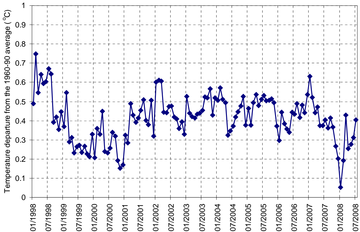
Figure 1: Evolution of the global temperature in the last ten years (data from CRU; combined land and marine temperatures; www.cru.uea.ac.uk/cru/data/temperature/hadcrut3gl.txt ).
