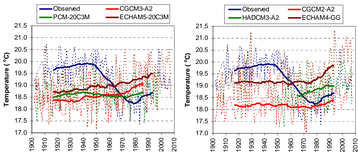
Figure 2: Plots of observed and GCM modelled annual (dotted lines) and 30-year moving average (continuous lines) temperature time series at Albany, USA (left AR4 models; right TAR models; reproduction of the original Fig. 5 from Koutsoyiannis et al., 2008, with kind permission of IAHS Press).
